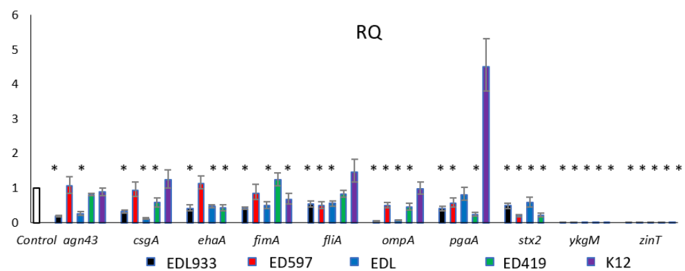
Figure 2. Expression levels of selected genes related to biofilm formation and pathogenesis in E. coli strains treated with or without C. martini EO at 0.05% ( v/v ) concentration. Transcriptional profiles were measured by qRT-PCR. * p < 0.01 .
