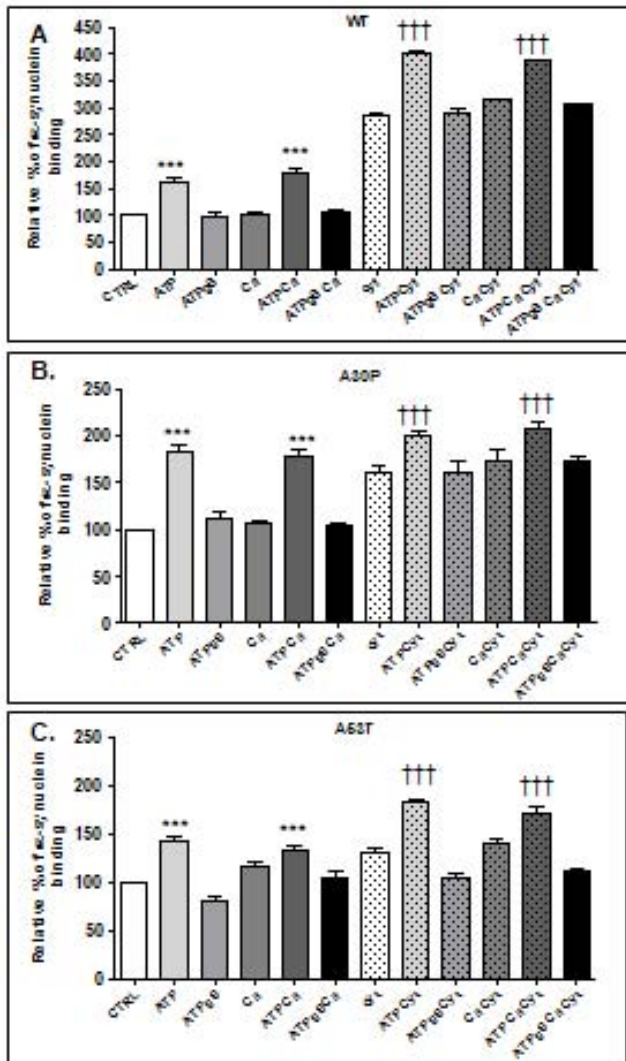
Figure 6 (A-C) Recombinant \alpha -syn (Wt, A30P and A53T) were incubated with ATP (1 mM), ATP \gamma S (3 mM), Ca 2+ (1 mM), ATP/Ca 2+ or ATP \gamma S/Ca 2+ in absence or presence of 1.5 mg/ml of KO cytosol, for 10 min at 37°C. Incubation with ATP (Student's T-test, p < 0.001 ), but not ATP \gamma S or Ca 2+ (Student's T-test, p > 0.05 ), induced a significant increase in the binding of Wt and mutant forms of \alpha -syn (compared to control condition without added cofactors).
