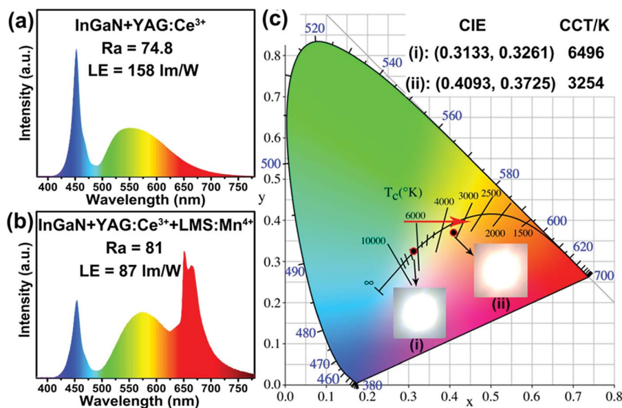
Fig. 5 EL spectra of the fabricated (a) cold WLED lamp (InGaN chip + YAG:Ce 3+ yellow phosphors) and (b) warm WLED lamp (InGaN chip + YAG:Ce 3+ yellow phosphors + LMS:Mn 4+ red phosphors) driven by 20 mA current. (c) CIE chromaticity diagram of the fabricated WLED lamps. The insets are photographs of the WLED lamps.
