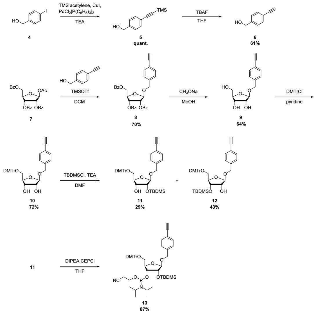
Scheme 2
