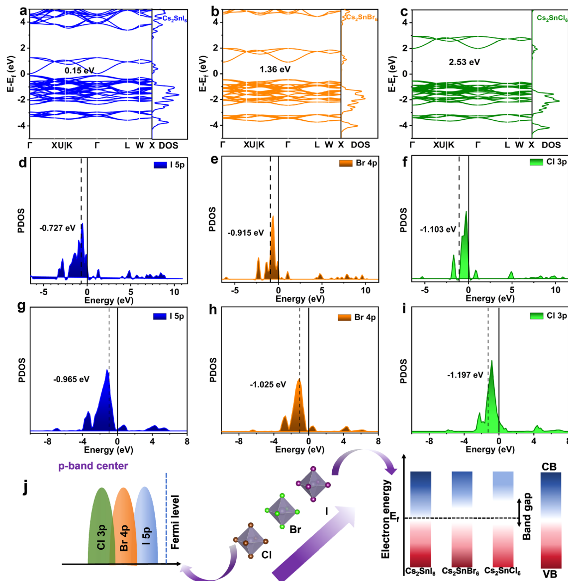
Fig. 1 DFT calculations of \text{Cs}_2\text{SnX}_6 ( X = \text{Cl}, \text{Br}, \text{I} ): electronic band structures of (a) \text{Cs}_2\text{SnI}_6 , (b) \text{Cs}_2\text{SnBr}_6 , and (c) \text{Cs}_2\text{SnCl}_6 . (d–i) PDOS files of (d and g) I 5p, (e and h) Br 4p, and (f and i) Cl 3p for (d–f) fresh \text{Cs}_2\text{SnX}_6 and (g–i) after adsorbing \text{Li}_2\text{S}_6 . (j) Schematic illustration of the p-band center regulation and electronic band structure of halide anions in \text{Cs}_2\text{SnX}_6 .
