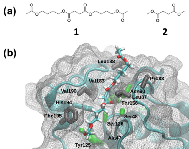
Figure 2. (a) PBS-like oligomer used as model substrate (compound 1) and dimethyl succinate (compound 2); (b) AoCut/1 Michaelis complex. The amino acid side chains in contact with compound 1 are shown as bold sticks (gray hydrophobic, green polar). The enzyme backbone is rendered as a cyan cartoon, while the enzyme surface as a gray wireframe.
