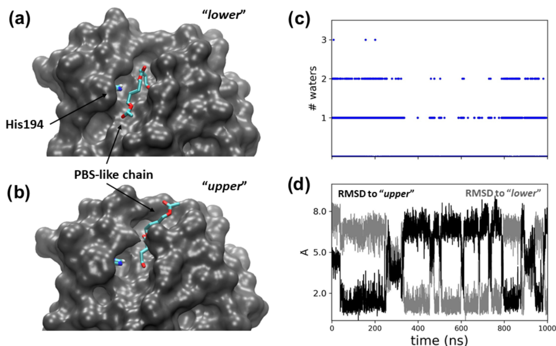
Figure 4. Acyl-enzyme intermediate. (a, b) Binding modes of the PBS-like chain in the active site cleft of AoCut; (c) the number of water molecule within 3.5 Å from the side chain of His194; (d) RMSD with respect to the two configurations shown in (a) (gray line) and (b) (black line).
