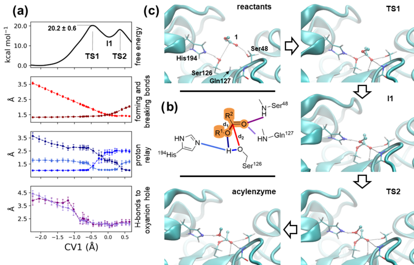
Figure 3. Acylation reaction step. (a) Free energy profile and relevant distances along the collective variable CV1 = d_1 - d_2 ; (b) chemical drawing highlighting the distances shown in panel (a); (c) representative configurations of reactants, transition states, and intermediate and acyl-enzyme states, labeled according to their corresponding CV1 values. For the sake of clarity, only the hydrolyzable moiety of compound 1 is drawn.
