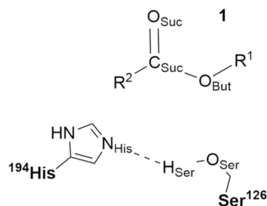
Scheme 1. Atom Labels Used to Describe the Acylation Step of the Hydrolysis of Compound 1 , a Poly(butylene succinate)-like Oligomer (Figures 1 and 2)
