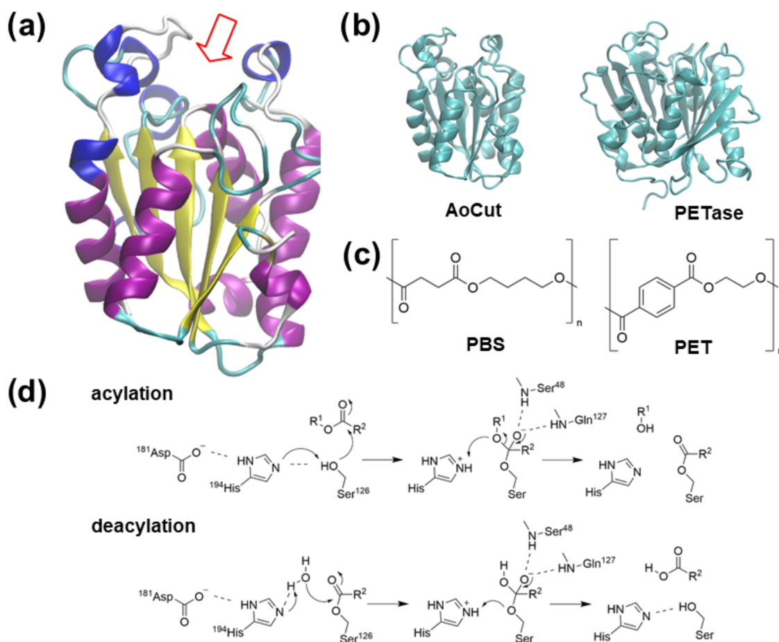
Figure 1. (a) Cutinase from A. oryzae (PDB ID: 3GBS); the red arrow points to the active site cleft; (b) AoCut and PETase share 16% sequence identity, and the common substructures display a RMSD of 3.2 Å; (c) chemical drawings of polyesters PBS and PET; (d) acylation and deacylation steps of the canonical esterase mechanism of ester hydrolysis.
