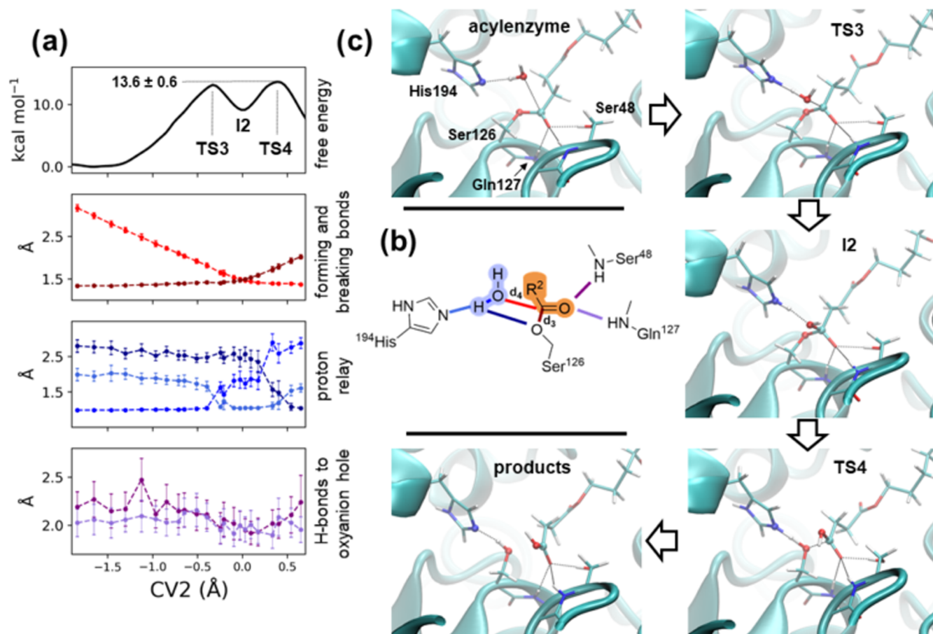
Figure 5. Decylation reaction step. (a) Free energy profile and relevant distances along the collective variable CV2 = d_3 - d_4 ; (b) chemical drawing highlighting the distances shown in panel (a); (c) representative configurations of reactants, transition states, and intermediate and product states, labeled according to their corresponding CV2 values.
