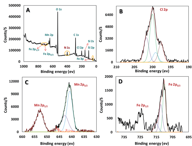
Fig. 4 The X-ray photoelectron spectroscopy (XPS) spectrum of catalyst ( \text{Fe}_3\text{O}_4@/\text{SiO}_2\text{-APTES-MnL}^{\text{GDC}} ).
