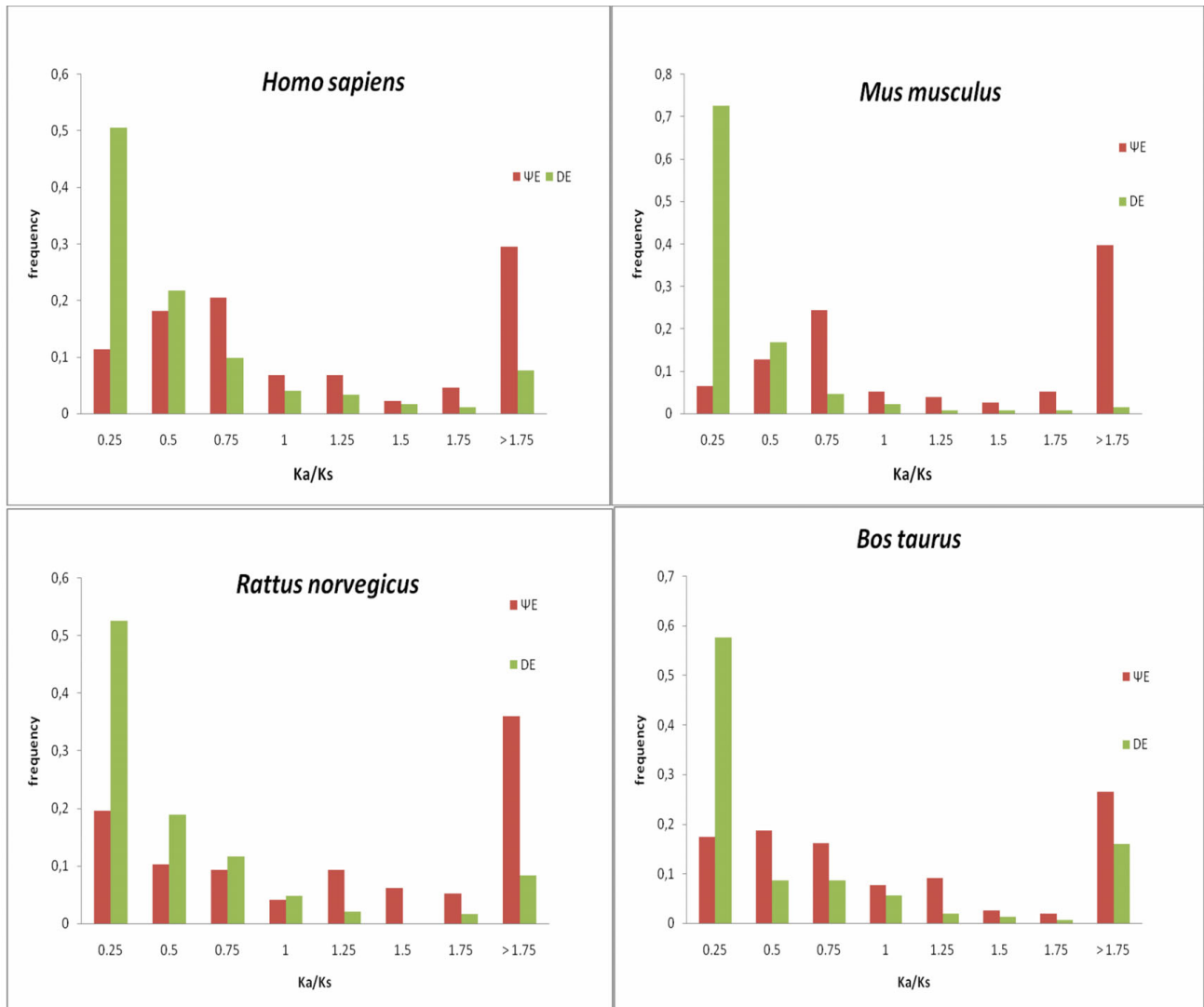
Figure 6 Histograms of K_a/K_s for DEs and ΨEs. The DE histogram is green, and the ΨE histogram is red. The bin label x is for all values such that, x-0.25 < \text{value} \leq x .
