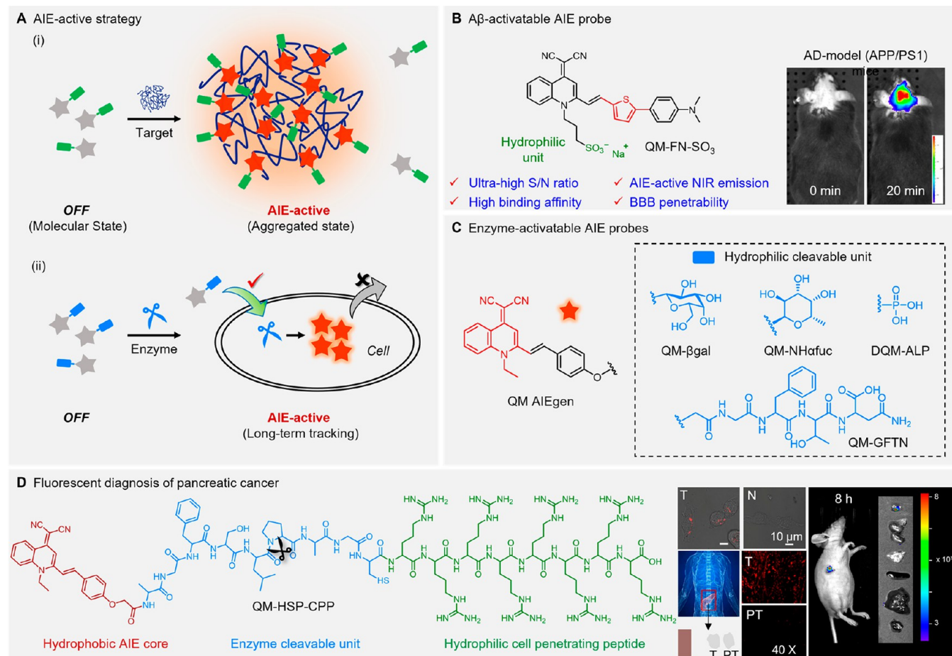
Figure 23. (A) AIE-active strategy. (B) QM-based \text{A}\beta probe QM-FN-SO 3 . Adapted with permission from ref 498. Copyright 2019 American Chemical Society. (C) Enzyme-activatable AIE probes: QM- \beta gal for \beta -galactosidase, QM-NHafuc for \alpha -lucosidase, DQM-ALP for hydrophilic alkaline phosphatase, and QM-GFTN for Atg4B protease. (D) QM-based probe QM-HSP-CPP for intraoperative pathological fluorescent diagnosis of pancreatic cancer via specific cathepsin E. Adapted with permission from ref 506. Copyright 2022 Wiley-VCH.
