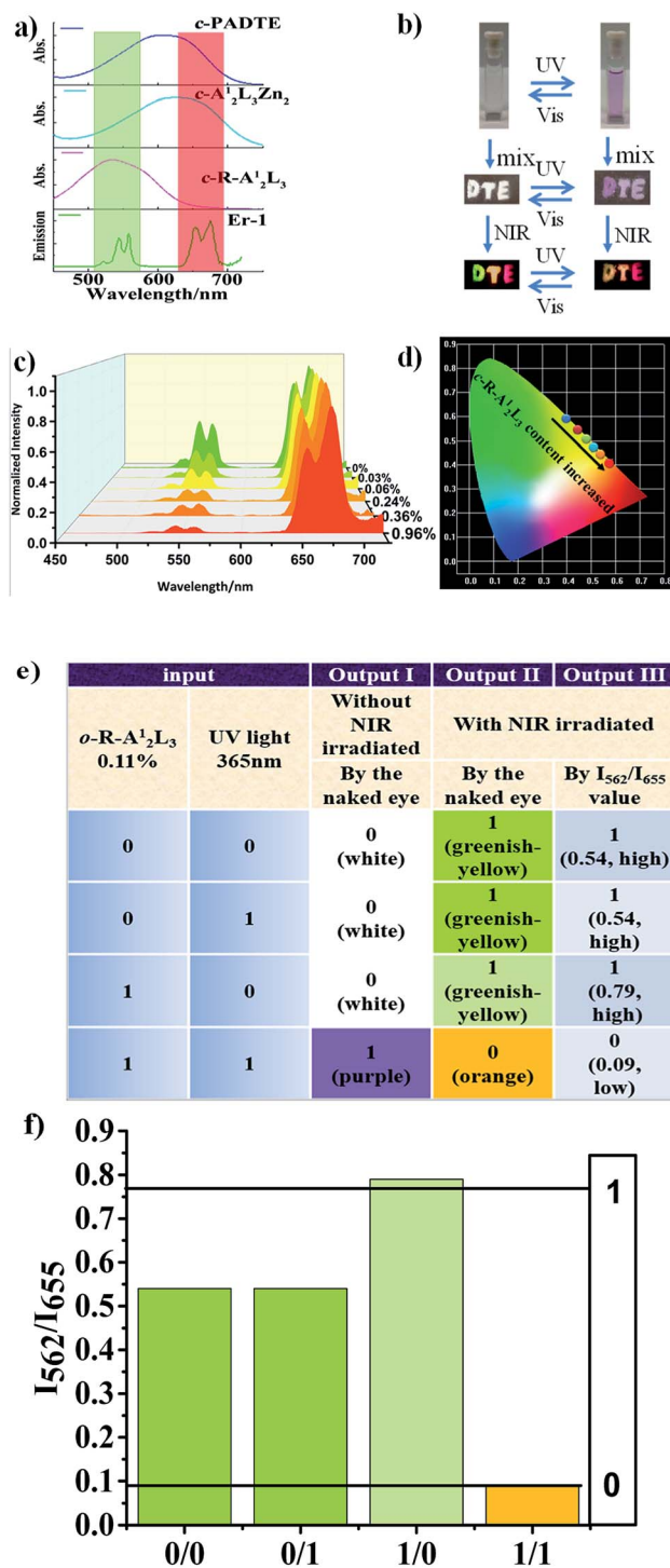
Fig. 5 (a) Overlap between the upconversion emissions of Er-1 and the UV-Vis absorption of c -PADTE, c - \text{A}_2^1\text{L}_3\text{Zn}_2 and c - \text{R-A}_2^1\text{L}_3 . (b) Color change processes by UV- or Vis-irradiation of o / c - \text{R-A}_2^1\text{L}_3 (upper), hybrid materials of \text{R-A}_2^1\text{L}_3 @Er-1 (for D), \text{R-A}_2^1\text{L}_3 @Er-5 (for T) and \text{R-A}_2^1\text{L}_3 @Er-9 (for E) under daylight (middle), and 980 nm-NIR excitation (lower). (c) Upconversion emission spectra and (d) CIE coordinates of hybrid materials by adding different ratios of c - \text{R-A}_2^1\text{L}_3 (0–0.96%). (e) The truth table for AND and NAND logic gates designed from the o - \text{R-A}_2^1\text{L}_3 -0.11%@Er-1 system and (f) the corresponding PL readout signals for output III.
