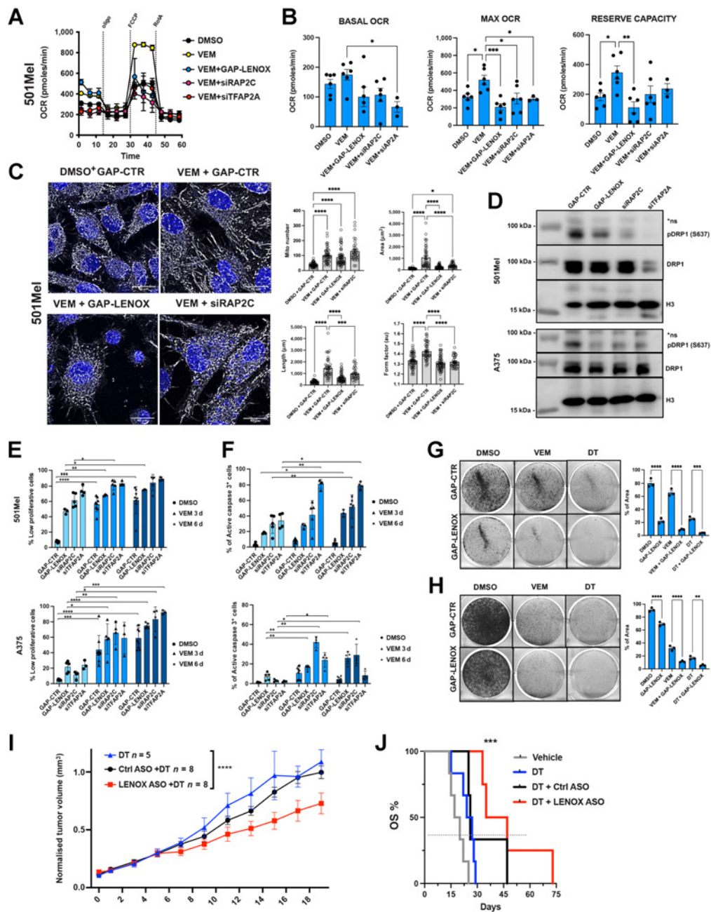
Figure 6. LENOX and RAP2C promote metabolic switch upon BRAF inhibition. A and B , Mito Stress Test of 501Mel cells grown for 3 days with DMSO or vemurafenib (1 µmol/L) and transfected as indicated. Experimental groups were compared by one-way ANOVA (Tukey test). C , MitoTracker CMXRos Red staining of cells treated with DMSO or vemurafenib, transfected as indicated and analyzed by confocal microscopy as in Fig. 4A . D , Phospho-DRP1 S637 and total-DRP1 levels in cells treated as above. H3 was used as loading control. E and F , Proliferation and apoptosis of cells treated as indicated. Experimental groups were compared by one-way ANOVA. G and H , Crystal violet staining of GapMeR-transfected cells. Percentages of occupied areas were compared by one-way ANOVA. I , Growth of MEL006res PDX in mice treated with DT with or without nontargeting ASO (DT+GAP-CTR) or LENOX-targeting ASO (DT+GAP-LENOX). Tumor size was measured daily for 20 days. Statistics were calculated using two-way ANOVA (Šidák multiple comparisons test). J , Kaplan-Meier plot showing overall survival (OS) of mice described in I . DT, n = 5 ; DT+GAP-CTR, n = 3 ; DT+GAP-LENOX ASO, n = 4 . Statistical analysis were calculated by log-rank (Mantel-Cox) test. *, P < 0.03 ; **, P < 0.002 ; ***, P < 0.0002 ; ****, P < 0.0001 .
