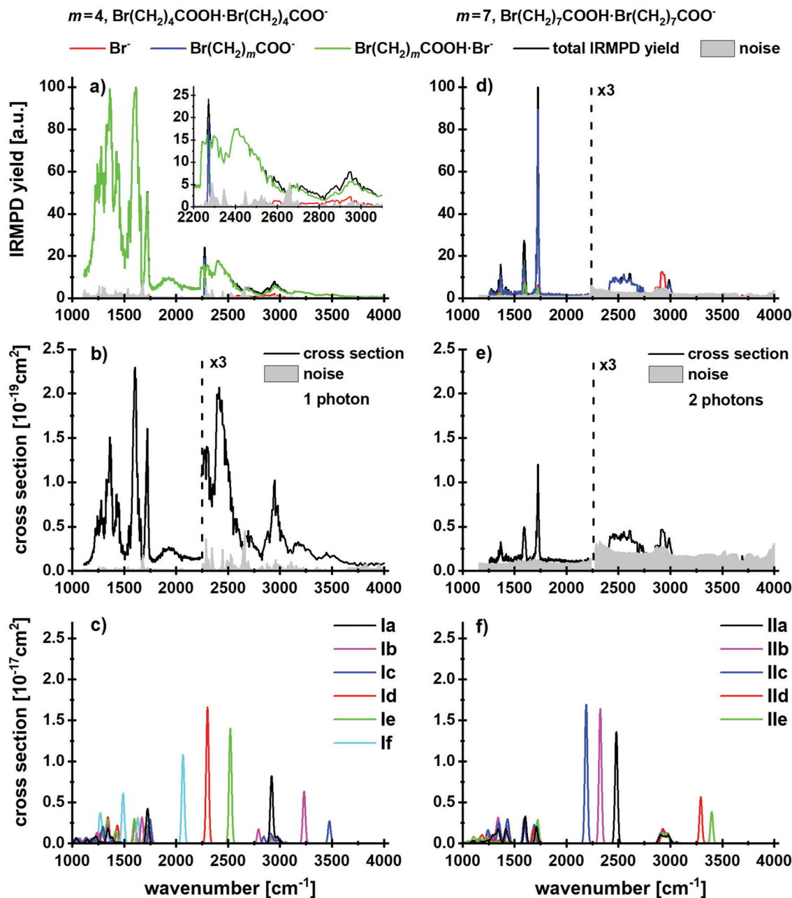
Fig. 1 (a and d) IRMPD yield spectra with the total yield (black line) and the corresponding fragment contributions (red, blue and green lines), (b and e) experimental and (c and f) theoretical cross sections of the cluster \text{Br}(\text{CH}_2)_m\text{COO}\cdot\text{Br}(\text{CH}_2)_m\text{COOH}\cdot\text{Br}^- with m = 4 and m = 7 . In (d), the \text{Br}^- and \text{Br}(\text{CH}_2)_7\text{COOH}\cdot\text{Br}^- fragments are superimposed at 1500–1750 \text{cm}^{-1} . Calculated at the B3LYP/def2TZVP level of theory.
