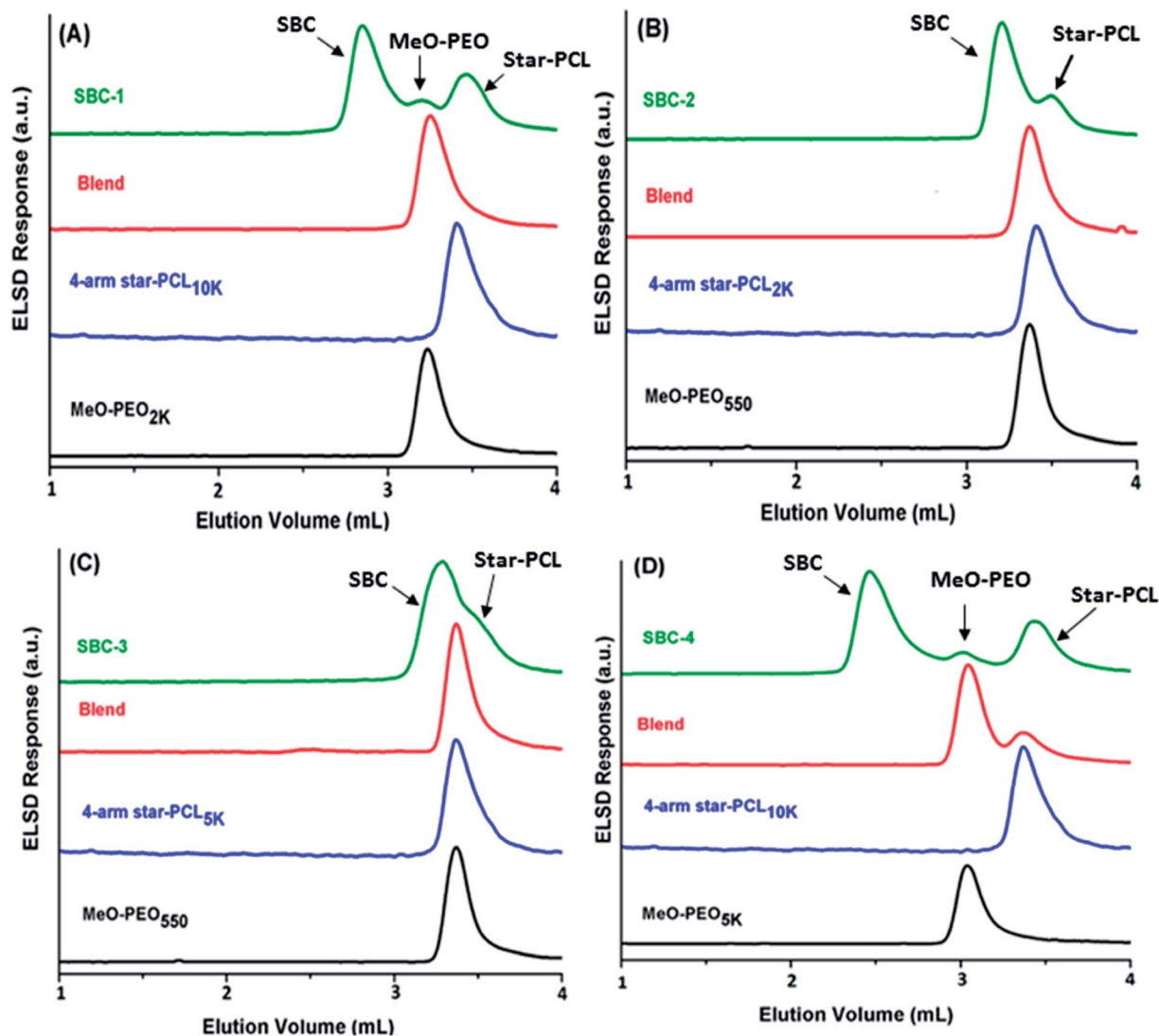
Fig. 8 Elutograms of (A) PCL 10k - b -PEO 2k -OMe; (B) PCL 2k - b -PEO 550 -OMe; (C) PCL 5k - b -PEO 550 -OMe; (D) PCL 10k - b -PEO 5k -OMe, and their respective blends at LCCC of star-PCL on stationary phase: Jupiter RP-C18; 250 × 4.6 mm; pore size: 300 Å, mobile phase (ACN/THF/TEA: 85/15/1, v/v), detection: ELSD.
