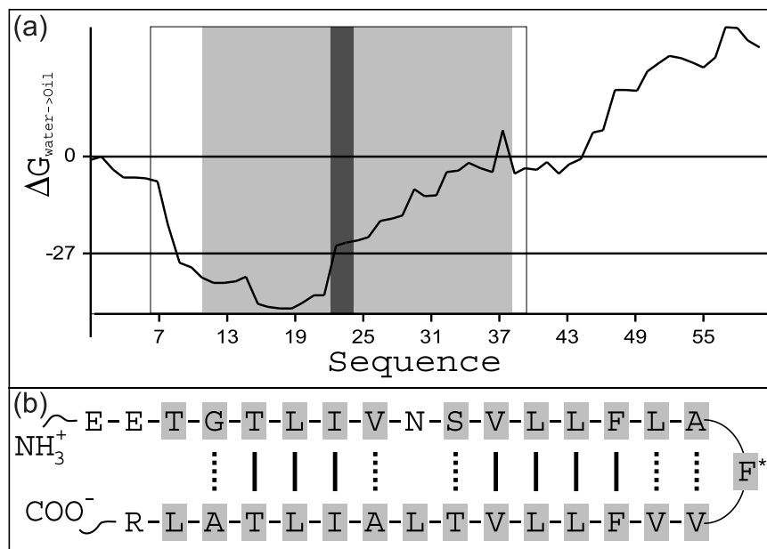
Figure 2. (a) Hydrophobicity analysis of the SCoV E protein according to the GES scale 28 using a window size of 15 and a hydrophobicity cutoff of \Delta G_{\text{water} \rightarrow \text{oil}} = -27 kcal/mol. 29 The region of the synthesized peptide is boxed, while gray shading indicates the extent of the hydrophobic stretch of the protein. The location of the iodinated Phe residue is indicated by dark shading. (b) Inversion diagram of the SCoV E protein hydrophobic region outlining identity and similarity between the two inverted sequence elements, in continuous and broken lines, respectively. Hydrophobic amino acid residues according to the GES scale 28 are indicated by gray shading.
