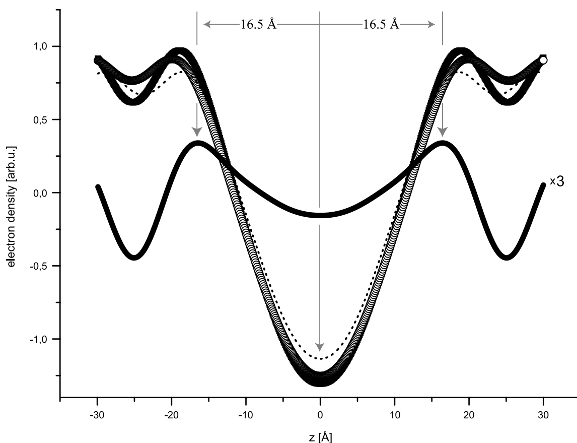
Figure 4. Electron density profile (on arbitrary scale around the mean density) of the lipid bilayers obtained at molar protein-to-lipid (DMPC/S-CoV E protein) ratios of P/L = 0.1 , for iodinated (filled symbols) and non-iodinated (open symbols) protein, as obtained from Fourier synthesis of measured integrated Bragg peak intensities. The difference between the two curves indicates the position of the one iodinated phenylalanine per protein located adjacent to the head-group region, close to the hydrophilic/hydrophobic interface. For comparison, the electron density profile of the Influenza A M2 H + channel transmembrane domain, a tetrameric helical bundle, 30 is depicted in broken line.
