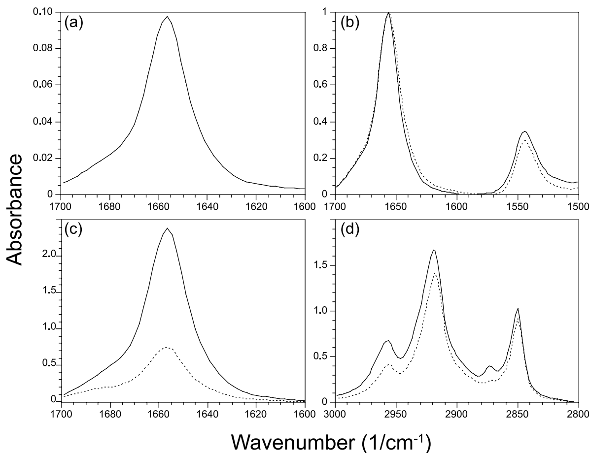
Figure 3. (a) Transmission FTIR spectrum of the SCoV E protein TMD reconstituted in DMPC lipid bilayers. (b) ATR-FTIR spectra of SCoV E protein TMD reconstituted in lipid bilayers, focusing on the amide I and amide II regions. Spectra were obtained after flushing air saturated with H 2 O (continuous line) or D 2 O (broken line) over the sample. Both spectra were normalized so as to adjust the absorption of the amide I mode to 1.0 OD. (c) ATR-FTIR spectra of SCoV E protein TMD reconstituted in lipid bilayers, focusing on the amide I region. Spectra were obtained with parallel (continuous line) or perpendicular (broken line) polarized light. (d) ATR-FTIR spectra as in c but focusing on the lipid CH 2 and CH 3 stretching modes.
