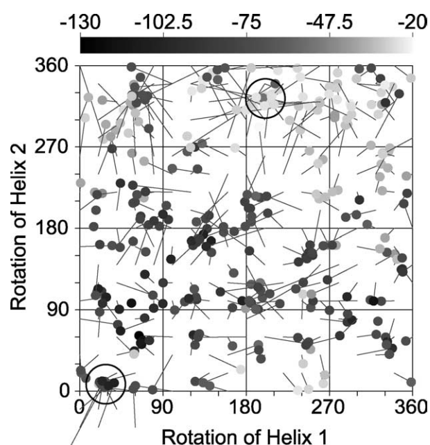
Figure 6. Results of the global searching molecular dynamics simulations of the two helices forming the hairpin of SCoV E protein. Each structure is positioned according to its final rotational angle of helix I and helix II, and colored according to energy of the bundle as indicated by the color legend (values in kcal/mol). The gray lines represent a vector connecting the starting position for each structure and the final one. The two single clusters found are encircled in the Figure.
