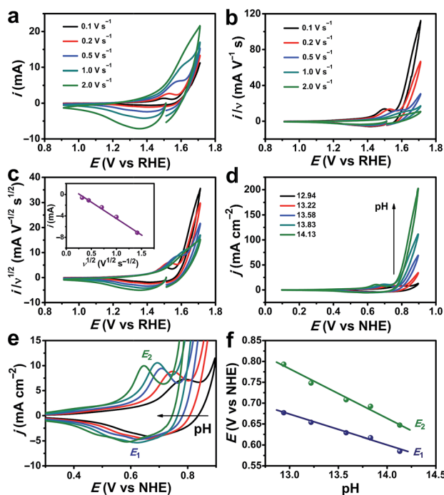
Fig. 6 (a–c) CV current–potential responses of P-400 at different scan rates. Inset in (c): i/\nu^{1/2} . (d) CVs of P-400 in different pH KOH solutions. (e) The enlarged part showing the CVs in (d). (f) The dependence of the precatalytic redox peak potentials E_1 and E_2 on pH.
