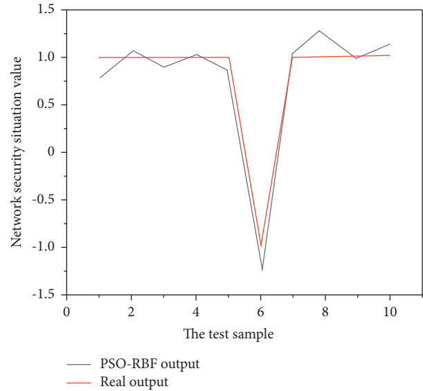
FIGURE 3: Comparison of PSO-RBF model prediction results and actual values.
