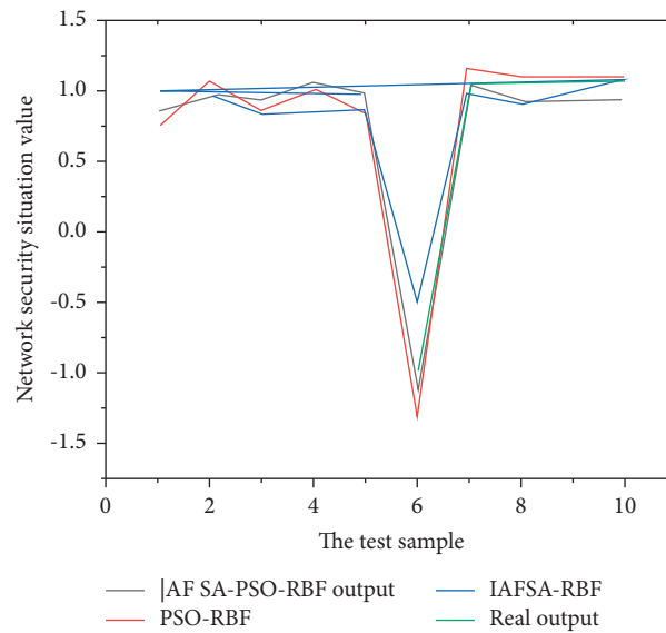
FIGURE 5: Comparison of the predicted results and actual values of the three models.
