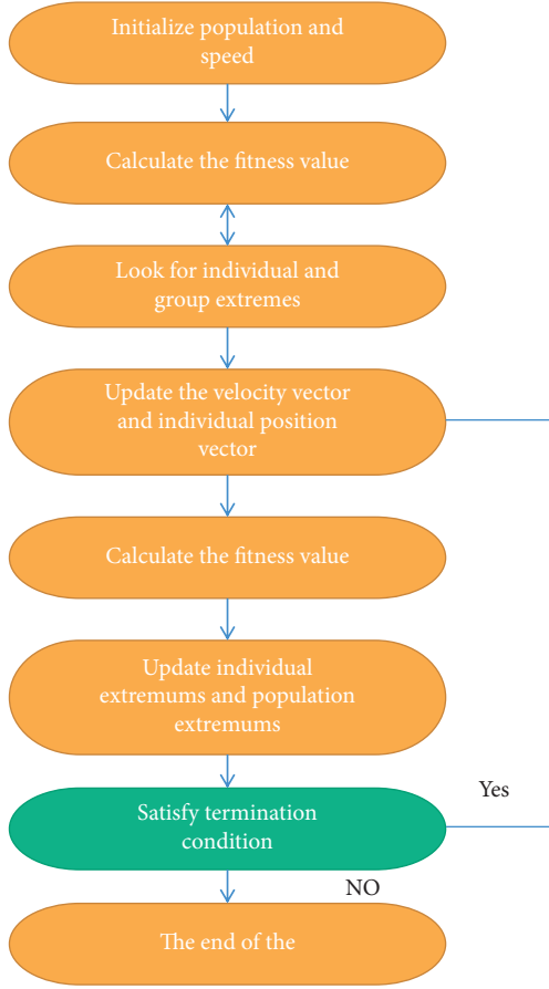
FIGURE 2: Flowchart of particle swarm algorithm.
