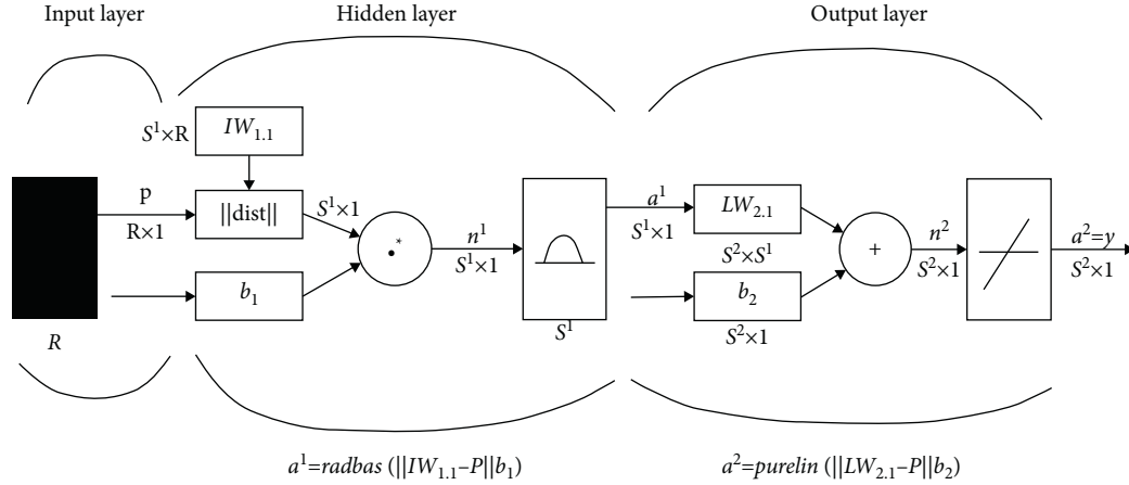
FIGURE 1: RBF neural network.
