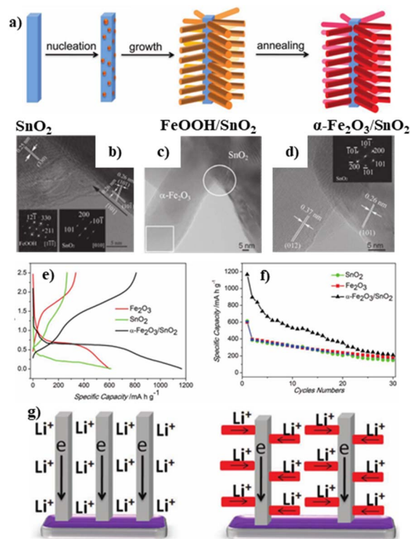
Fig. 7 (a) Scheme showing the formation process of α-Fe 2 O 3 /SnO 2 heterostructures; HRTEM image of (b) FeOOH/SnO 2 , (c and d) α-Fe 2 O 3 /SnO 2 ; (e) first charge–discharge profiles at a current density of 1000 mA g -1 ; (f) cycling performance of different samples; (g) schematic comparison of the unidirectional nanowires and branched nanostructures for Li and electron transfer. Reproduced with permission from ref. 49. © Wiley-VCH GmbH, 2011.
