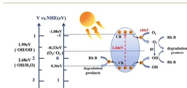
Fig. 9 Schematic diagram of the charge transfer and separation in the compound 2 and possible mechanism of its photocatalytic degradation of RhB under simulated sunlight irradiation.
