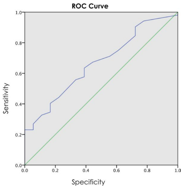
FIGURE 1. The ROC curve for the phase angle.
