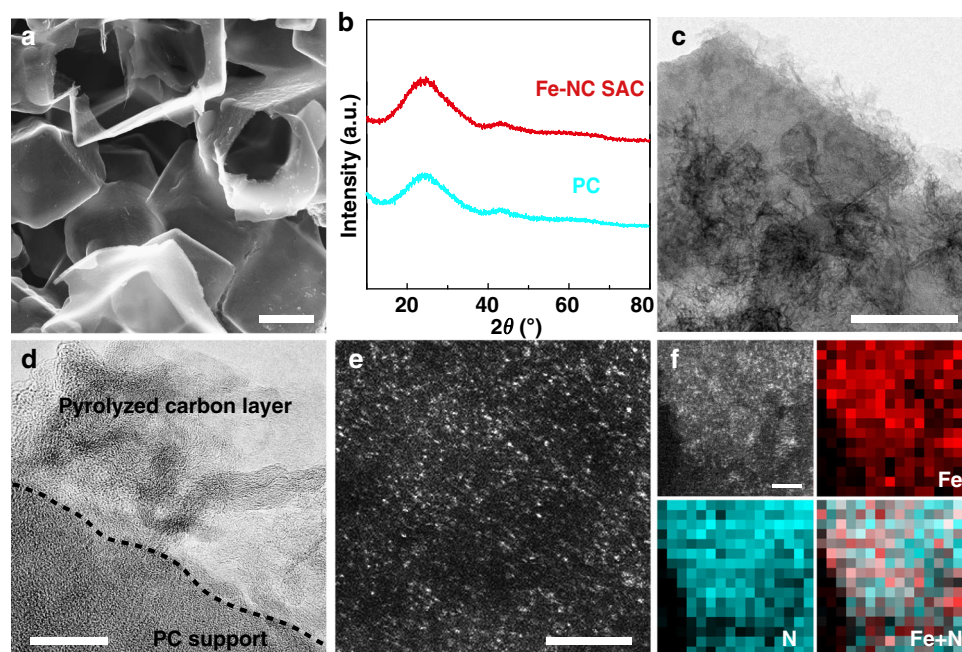
Fig. 2 Structural characterizations of PC support and \text{Fe-NC} SAC. a SEM image of PC support. b XRD patterns of PC and \text{Fe-NC} SAC. c TEM, d , HRTEM, e , HAADF-STEM images of \text{Fe-NC} SAC. f HAADF-STEM image and EELS mapping images of Fe, N, and overlaid Fe and N on \text{Fe-NC} SAC. Scale bars, 1 \mu\text{m} ( a ); 200 \text{ nm} ( c ); 20 \text{ nm} ( d ); 3 \text{ nm} ( e ); 2 \text{ nm} ( f )
