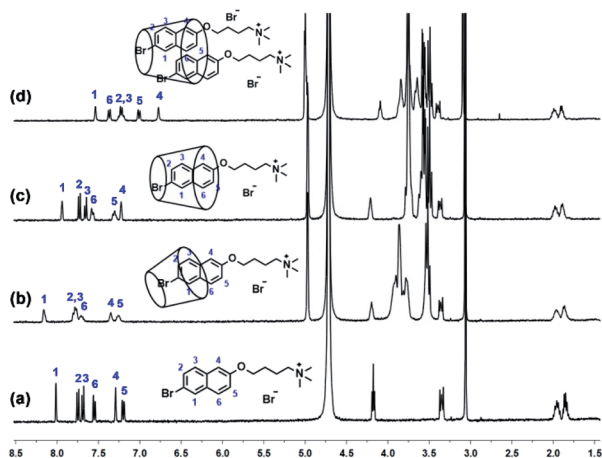
Fig. 1 ^1\text{H} NMR (400 MHz, \text{D}_2\text{O} , 298 K) spectra of 4C (a) after adding 1.0 equivalent \alpha -CD (b), \beta -CD (c), and \gamma -CD (d). ( [\text{4C}] = [\alpha\text{-CD}] = [\beta\text{-CD}] = [\gamma\text{-CD}] = 2 \text{ mM} ).
