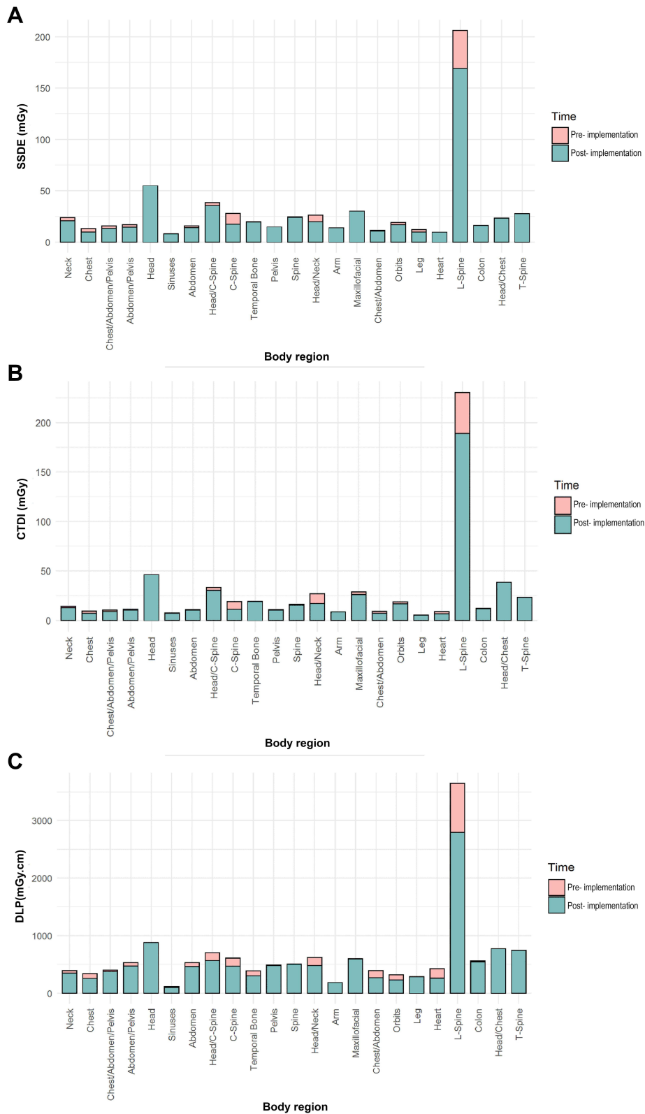
Figure 2 CT indices pre- and post-implementation of corrective measures based on imaged body region. SSDE (A), CTDI (B), and DLP (C). Overlapping bars from both time points indicate the difference in exposure between the two time points.
