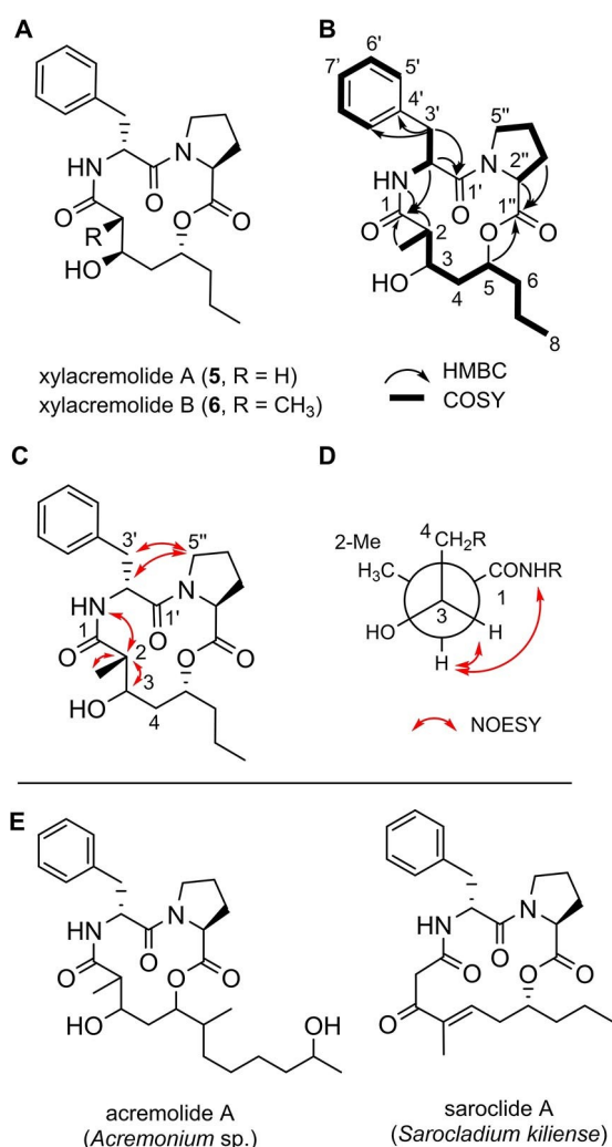
Figure 3. A) Structures of xylacremolide A ( 5 ) and B ( 6 ). B) Key COSY and HMBC, C) NOESY correlations and D) Newman projection of 2-Me (C2–C3 bond) to determine stereochemical assignment of 5 and 6 . E) Structures of related natural products.
