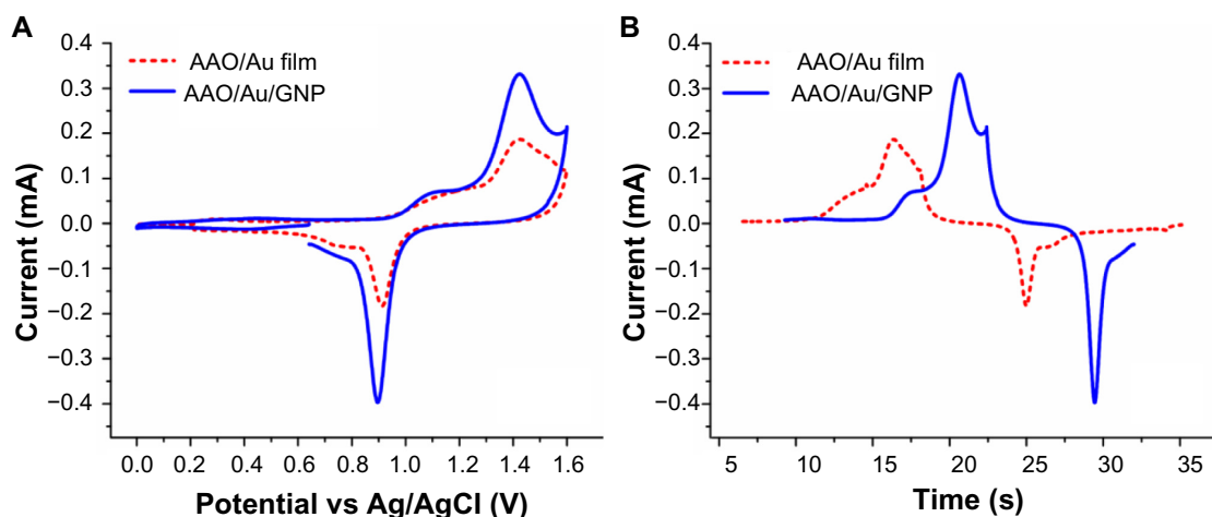
Figure 4 Cyclic voltammogram for the AAO/Au thin film electrode and the AAO/Au thin film/GNP electrode in a solution of 20 mM K_3Fe(CN)_6 with 0.1 M KCl as the supporting electrolyte; (A) I - V curve (B) I - t curve.
