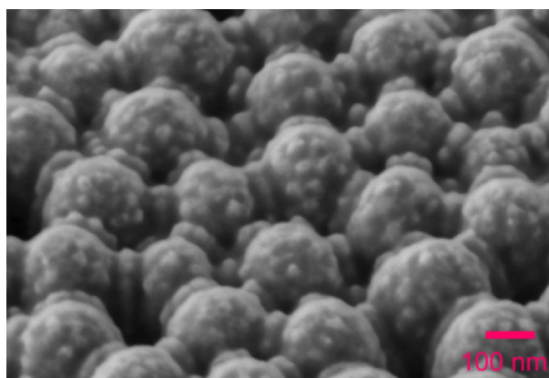
Figure 3 Scanning electron microscopic image of the GNP-deposited nanostructured electrode.
