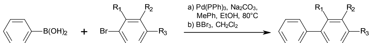
Figure 1 Synthesis and chemical structure of 2OH-CB3, 3OH-CB3 and 4OH-CB2.
