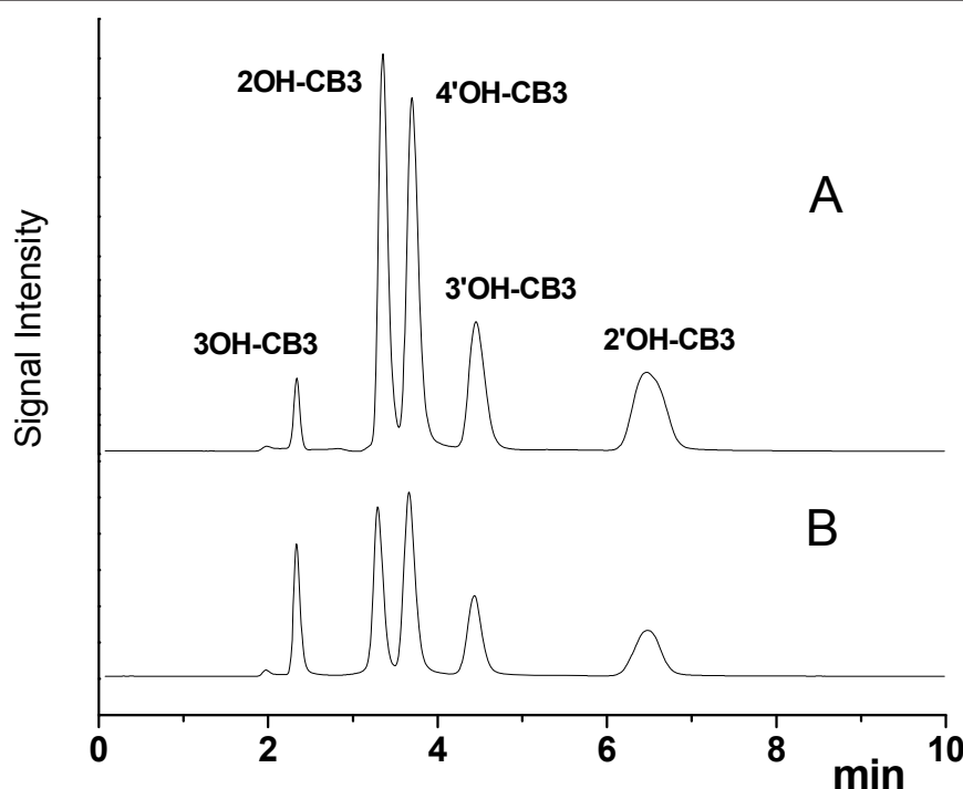
Figure 2 Chromatograms of five OH-CB3s in the root sample and standard. A: root sample; B: standards of five OH-CB3s.
