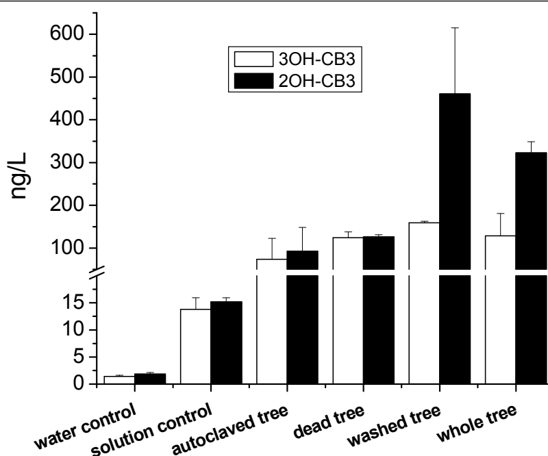
Figure 4 A comparison of 2OH-CB3 and 3OH-CB3 concentrations ( n = 3 ) in the solutions without poplars (deionized water control and hydroponic solution control) and with poplars (autoclaved poplar, dead poplar, washed poplar and whole poplar) after 10 days' exposure to a spiked concentration of 1.0 \text{ mg L}^{-1} CB3.
