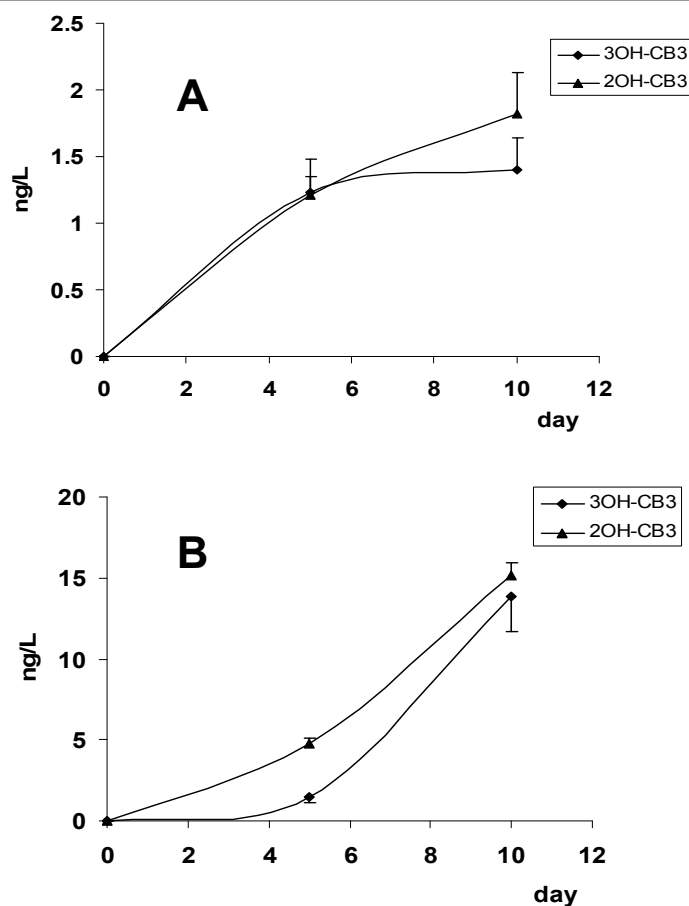
Figure 3 Abiotic Controls of deionized water (A) and hydroponic solution (B). Concentrations of 2OH-CB3 and 3OH-CB3 (n = 3) developed over 10 days following an initial concentration spike of parent compound CB3 at a concentration of 1.0 mg L -1 .
