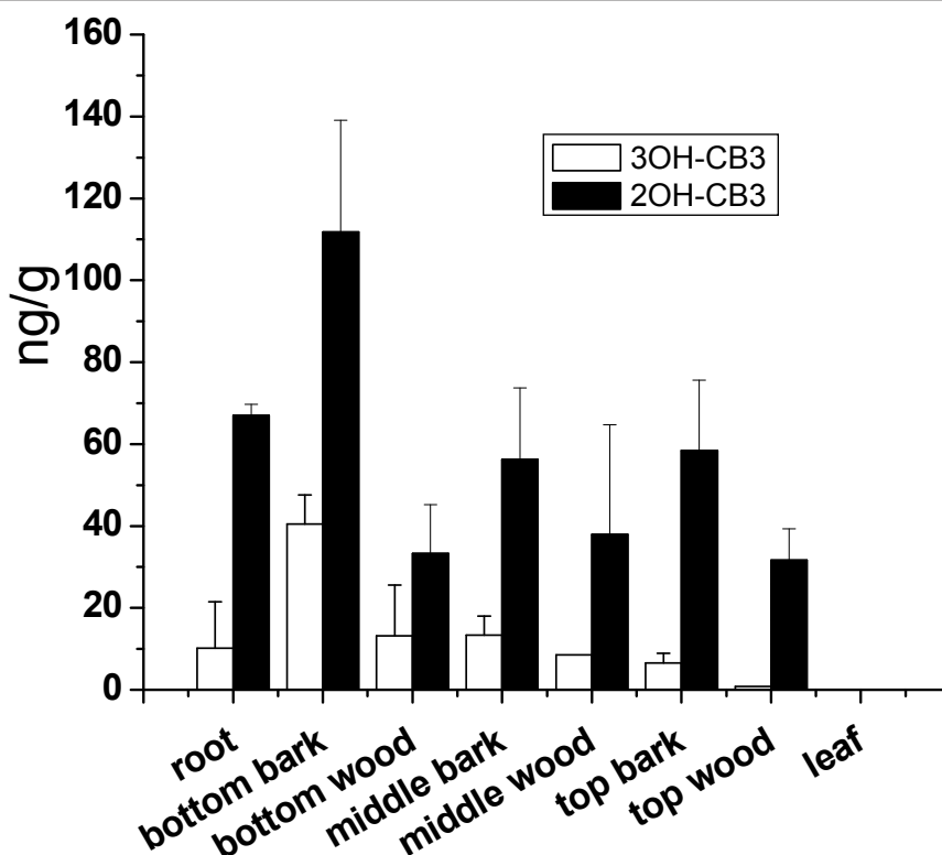
Figure 5 A comparison of 2OH-CB3 and 3OH-CB3 concentrations ( n = 3 ) in the different parts of a whole poplar plant after 10 days' exposure (an initial concentration spike of parent compound CB3 was added on day zero at a concentration of 1.0 \text{ mg L}^{-1} ).
