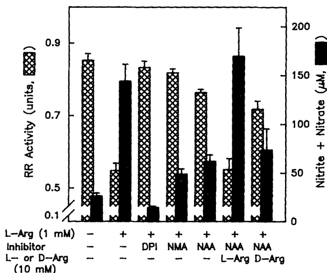
Figure 2. Inactivation of RR by NO synthase in lysates of activated macrophages. Partially purified RR (5 mg protein/ml) was incubated with NO synthase from activated macrophages (4 mg protein/ml) in the presence of Mn-superoxide dismutase (200 U/ml), catalase (1,000 U/ml), 0.25 mM NADPH, 4 \mu M tetrahydrobiopterin, and 4 \mu M FAD. L-Arginine (1 mM), diphenyleneiodonium (DPI, 10 \mu M), N ω -methyl-L-arginine (NMA, 0.5 mM), N ω -amino-L-arginine (NAA, 0.5 mM), and excess L- or D-arginine (10 mM) were further added as indicated. After incubation for 45 min at 37°C, RR activity was measured. Cross-hatched bars indicate RR activities; solid bars indicate the concentration of nitrite plus nitrate generated. Bars and brackets indicate the mean and SD of triplicates.
