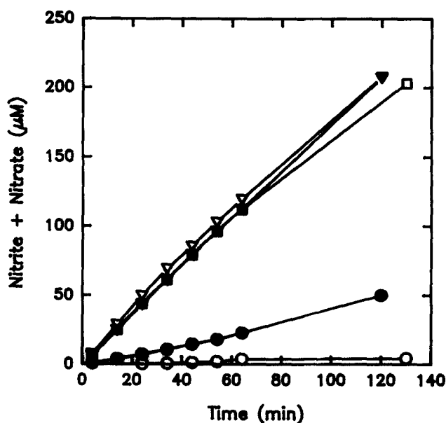
Figure 4. Oxidation of hydroxyurea to nitrite/nitrate. Hydroxyurea (1 mM) was incubated with varying concentrations of CuSO 4 ( \circ , no addition; \bullet , 1 \mu M; \nabla , 5 \mu M; \blacktriangledown , 10 \mu M; \square , 20 \mu M) in the presence of 1 mM H 2 O 2 in 2.5 mM sodium phosphate, pH 7.5, at 37°C. After the indicated periods of incubation, samples were analyzed for nitrite plus nitrate.
