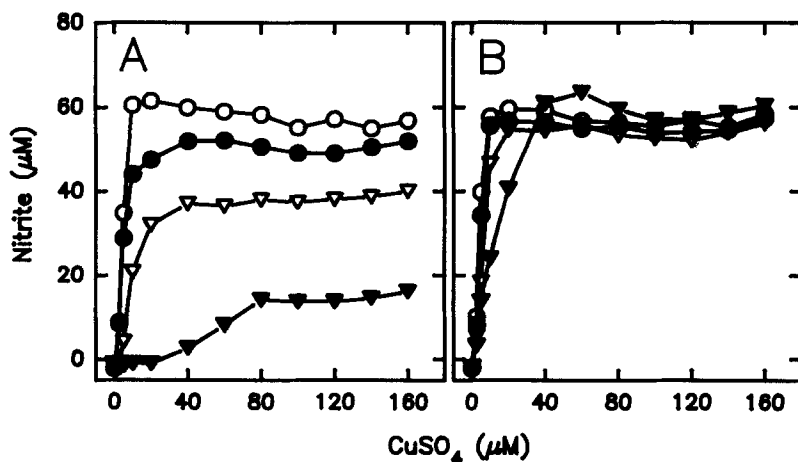
Figure 5. Inhibition of nitrite production from hydroxyurea by ferredoxin but not by albumin. The ability of \text{CuSO}_4 at the indicated concentrations and \text{H}_2\text{O}_2 (1 mM) to generate nitrogen oxides from hydroxyurea (0.3 mM) was examined without further additions (O) or in the presence of Clostridium pasteurianum ferredoxin (A) or BSA (B) at concentrations of 0.1 mg/ml ( \blacktriangledown ), 0.01 mg/ml ( \nabla ), or 0.001 mg/ml ( \bullet ). After a 60-min incubation at 37^\circ\text{C} , the reaction was stopped by adding EDTA (0.1 mM) and catalase (1,000 U/ml), and the concentration of nitrite was measured. Data are the means of duplicates.
