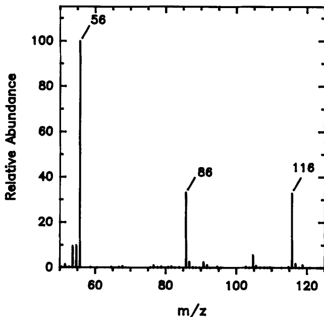
Figure 6. Mass spectrum of nitrosomorpholine generated from the oxidation of hydroxyurea in the presence of morpholine. Oxidation of hydroxyurea (0.3 mM) with 10\ \mu\text{M} \text{CuSO}_4 and 2 mM \text{H}_2\text{O}_2 was carried out in the presence of 10 mM morpholine to trap generated NO. The reaction mixture was extracted with dichloroethane, concentrated under \text{N}_2 , and analyzed by GC/MS. A peak eluting at 3.8 min showed a molecular ion of m/z 116 and base fragment ion of m/z 56.
