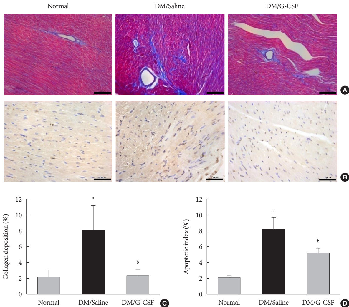
Fig. 3. Granulocyte-colony stimulating factor (G-CSF) improves fibrosis and apoptosis in a rat model of diabetic cardiomyopathy. (A) Representative images of Masson's trichrome (MT) staining of heart tissue at 4 weeks after treatment in each group ( \times 200 ). (B) Representative photomicrographs showing terminal deoxynucleotidyl transferase dUTP nick end labeling (TUNEL) assay staining in the myocardium at 4 weeks after treatment in each group ( \times 200 ). Scale bar = 100 \mu\text{m} . (C) Results of quantitative analysis of collagen area as a ratio of fibrotic area to heart area. (D) Results of quantitative analysis of apoptotic cells. All data are expressed as mean \pm standard error ( n=8 per group). DM, diabetic rat model. a P<0.05 vs. normal, b P<0.05 vs. DM/saline.
