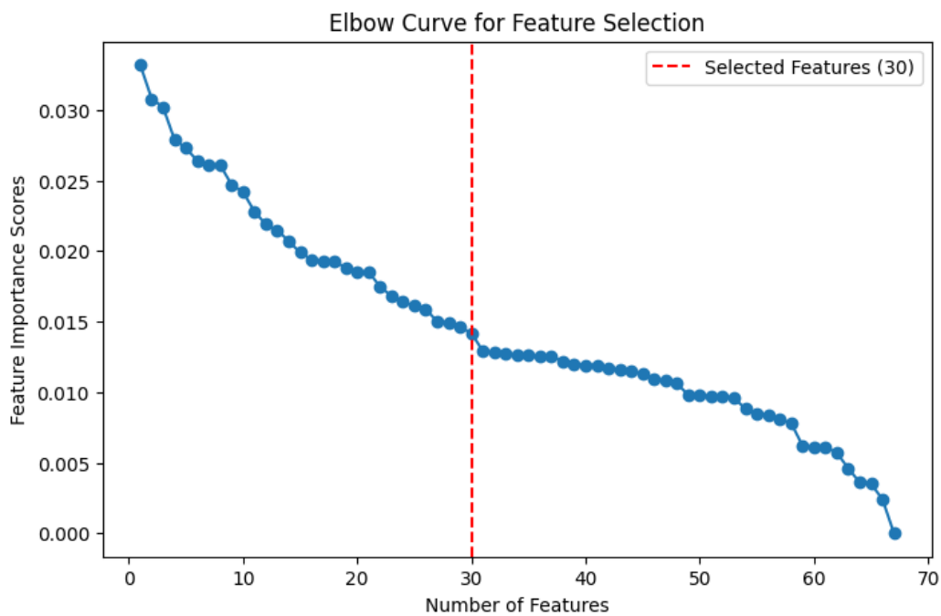
Supplementary Figure 2. Elbow plot for the second use case.
