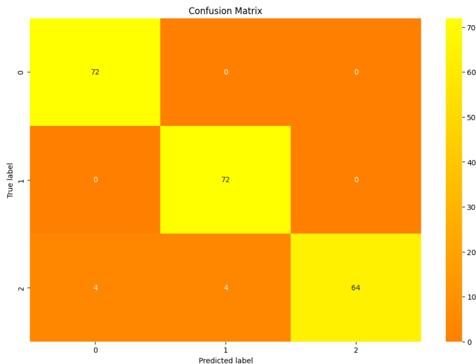
Supplementary Figure 1. Confusion matrix of the best performing algorithm of the FCM analysis of the first use case.
