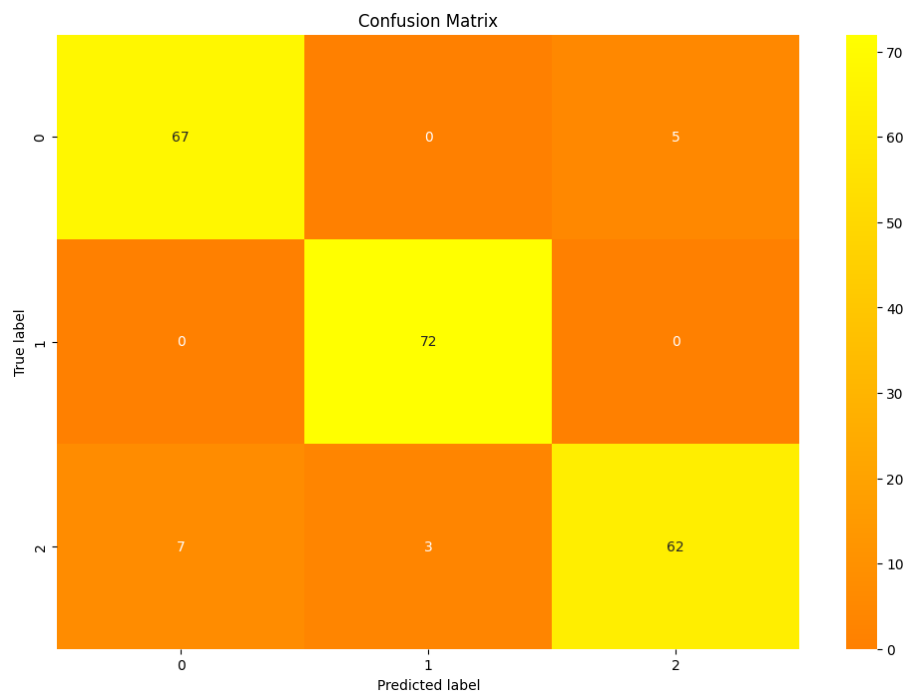
Supplementary Figure 2. Confusion matrix of the best performing algorithm of the FCM analysis of the second use case.
