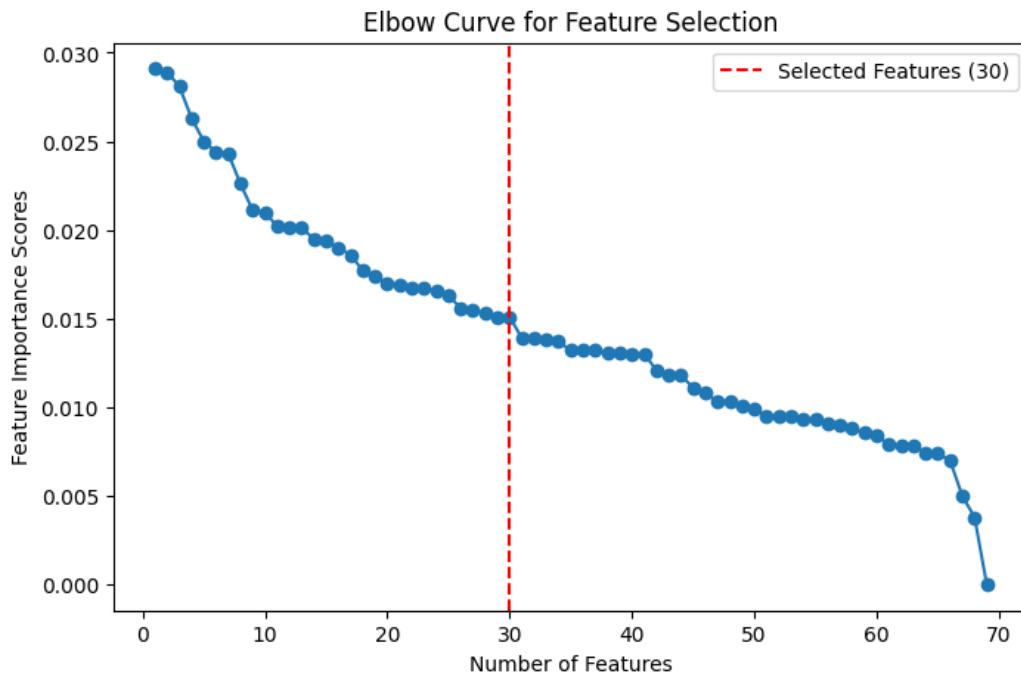
Supplementary Figure 1. Elbow plot for the first use case.
