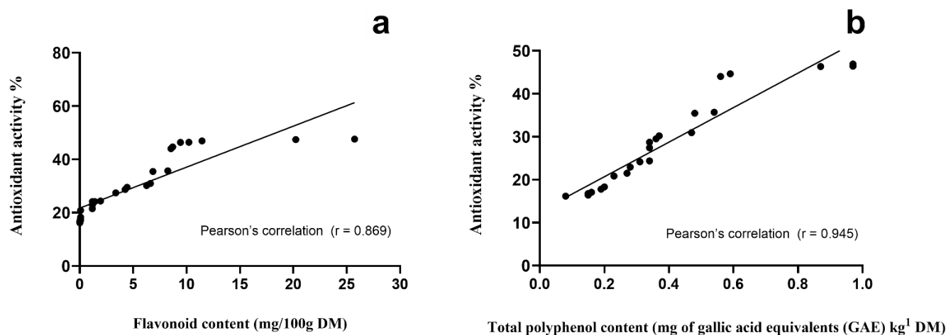
Figure 1. Pearson's correlations of flavonoid (a) and total polyphenol (b) content versus antioxidant activity of vegetation species browsed/grazed by goats on semiarid rangelands.
