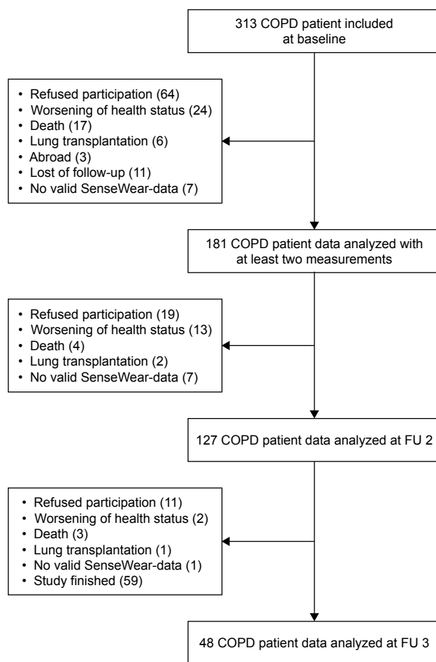
Figure 1 Study flow.
