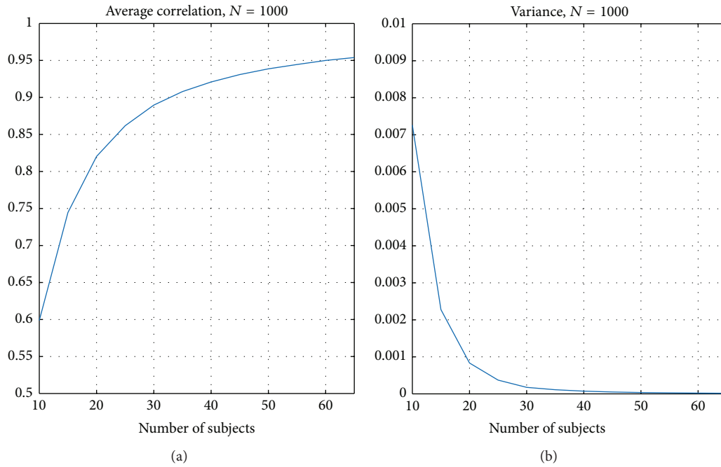
FIGURE 2: Average correlation C_{avg} over 1000 resampling replications. (a) presents the average correlation over and (b) the corresponding variance of C_n , n = 1, \dots, 1000 . The correlation increased when the sample size increased and at the same time the variance decreased.
