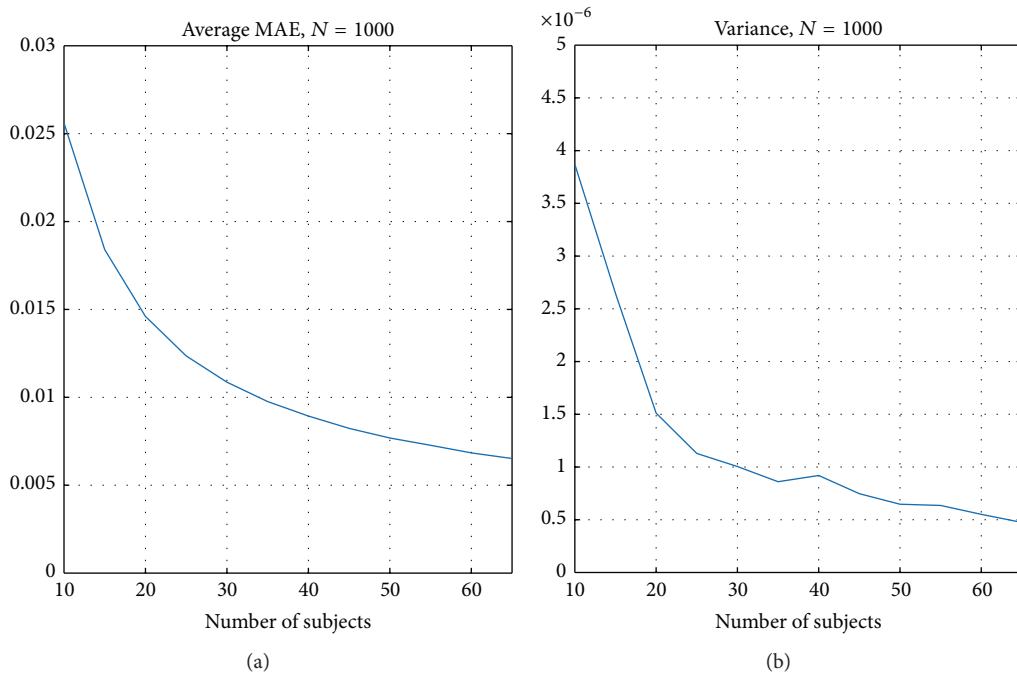
FIGURE 3: Average MAE M_{avg} over 1000 resampling replications. (a) presents the average MAE and (b) the corresponding variance of M_n , n = 1, \dots, 1000 .
