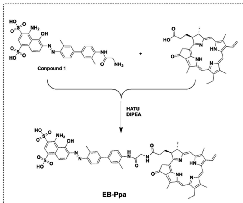
Scheme 1 The structure and synthesise route of probe EB-Ppa.
