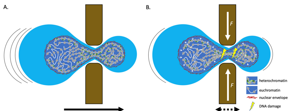
Figure 2. Chromatin dynamics during migration. (A) When a cell migrates (black arrows) through a small space, resulting in extensive compression of the cellular interior, chromatin tends to become hyper condensed. As we predict that heterochromatin is more gel-like than euchromatin, this might facilitate the nucleus to move through the gap faster, in a capillary suction-like manner. (B) When a cell is exposed to extensive compression forces (white arrows) or is stuck in a gap, the chromatin will eventually detach from the nuclear envelope and becomes more susceptible to DNA damage. This supports a model where chromatin-nuclear envelope contact serves to protect the DNA in a multi-contact manner. Intriguingly, dual functions for DNA repair factors have been observed. In addition to facilitating DNA repair, some DNA-repair factors have non-DNA repair functions. ATR that is localized to the nuclear periphery relocates upon osmotic stress and mechanical stretching, regulating chromatin condensation and nuclear envelope breakdown [56–58]. A deep mechanistic dissection of how DNA damage is repaired under force regimens will be extremely important, as well as how the DNA repair machinery manages mechanical forces.
