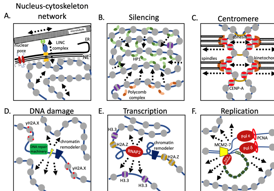
Figure 3. Nuclear machinery alter chromatin properties. (A) Physical forces are transmitted to the chromatin through a trans-nuclear envelope protein complex, altering both chromatin compaction and gene transcription. (B) Gene repression is commonly achieved through heterochromatin formation by either HP1 or Polycomb complexes, resulting in chromatin condensation and reduced chromatin elasticity. (C) Mitosis is a highly physical event, where in a highly coordinated manner, chromosomes are moved over extensive distances through the mitotic spindle machinery. The pushing and pulling forces that are exerted on the chromosomes, and especially the centromeric chromatin, are critical in satisfying the spindle checkpoint. (D) DNA damage must be repaired as quickly as possible, recruiting the DNA repair machinery, and locally decondensing chromatin, temporarily altering the local chromatin dynamics in part by enrichment of phosphorylated H2A.X nucleosomes. (E) Gene transcription is one of the most profound events in the nucleus, where the transcriptional machinery distorts the DNA double helix both behind and in front of the RNA polymerase. Highly transcribed regions are also enriched for H2A.Z and H3.3 nucleosomes. These nucleosomes might alter the local chromatin properties, potentially bringing together distant sites, such as enhancers and promoters. (F) Replicating chromatin has to decondense for the replication machinery to pass through, while at the same time maintaining distinct chromatin marks to be present on both newly formed strands. This highly dynamic and local event might temporarily increase the chromatin's elasticity. ER = endoplasmic reticulum, NE = nuclear envelope.
