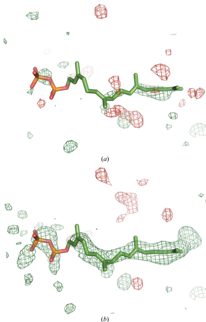
Figure 10 ( a ) Simulated-annealing OMIT map and ( b ) polder map for ligand GRG 502 in PDB entry 4opi. The positive and negative mF_{\text{obs}} - DF_{\text{model}} OMIT difference density contoured at 3\sigma is displayed in green and red, respectively.
