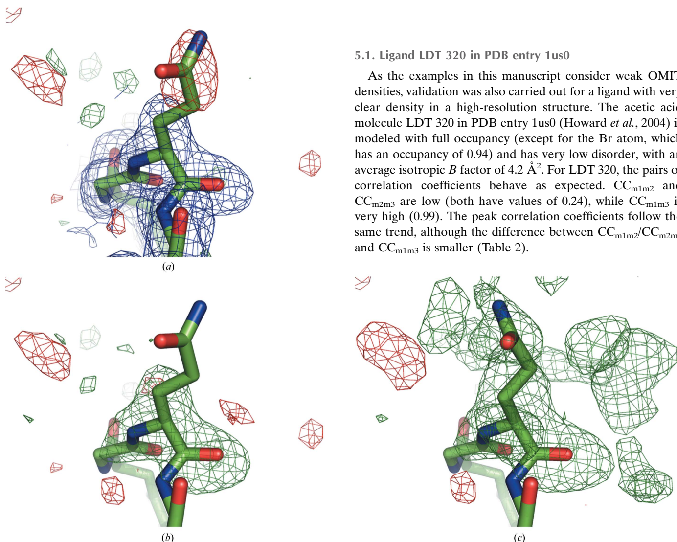
Figure 7 (a) Original 2mF_{\text{obs}} - DF_{\text{model}} (blue, 1\sigma contour) and mF_{\text{obs}} - DF_{\text{model}} maps, (b) OMIT map and (c) polder map for residue GlnH105 in structure 1f8t. The positive and negative mF_{\text{obs}} - DF_{\text{model}} difference density contoured at 3\sigma is displayed in green and red, respectively. In (c), the Gln side chain was real-space refined in Coot .
