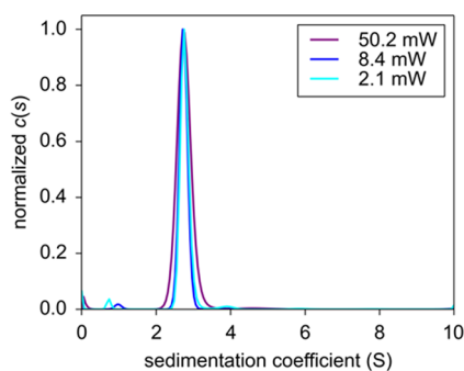
Figure 2. Sedimentation coefficient distributions c(s) corresponding to the fits of the FDS-SV data of Dronpa in Figure 1.
