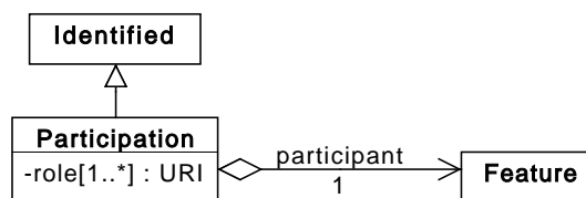
Figure 13: Diagram of the Participation class and its associated properties.
