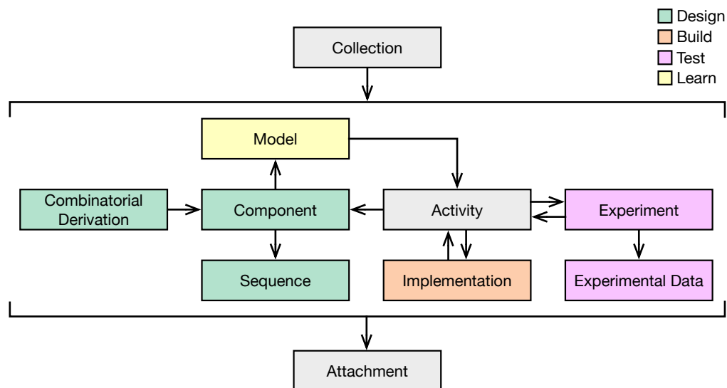
Figure 3: Main classes of information represented by the SBOL 3 standard, and their relationships. Green boxes represent design classes, orange boxes represent build classes, purple boxes represent test classes, yellow boxes represent learn classes, and the gray boxes represent additional utility classes. Each of these classes will be described in more detail below.
