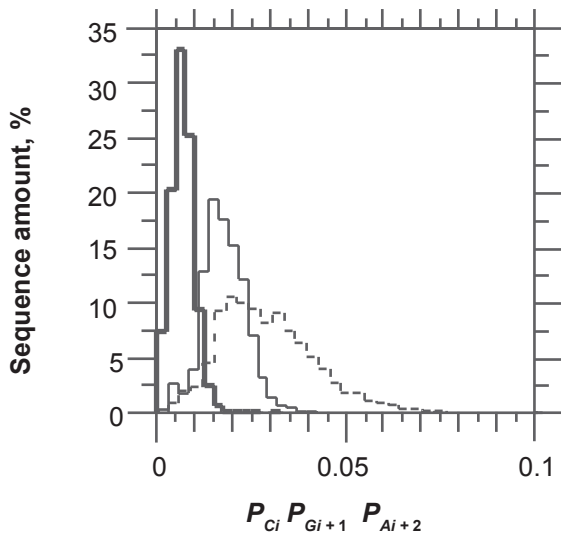
Figure 3. Distribution of P_{C_1}P_{G_1+1}P_{A_i+2} (bold), P_{G_1}P_{A_2}P_{C_3} (dashed) and P_{A_1}P_{C_2}P_{G_3} (thin) in the coding sequences of O. sativa , A. thaliana , H. sapiens , D. melanogaster , C. reinhardtii and P. falciparum grouped together.
