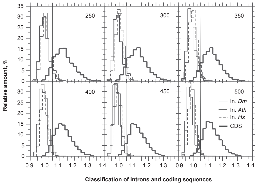
Figure 6. Classification of coding sequences (CDS) and introns (In) between 250 and 500 bp and among the six frames. The intron distributions of A. thaliana ( Ath , plain), D. melanogaster ( Dm , thin) and H. sapiens ( Hs , dashed) are centered on the classification value of 0.95. The CDS distribution of the six species grouped together (bold) are centered on the classification value of 1.10. The plain line (vertical) is for the threshold of classification of introns and CDSs at 1.05. The classification function was C=f_1+f_3+f_4 below GC = 55% and C=f_1+f_3+f_4+f_5 above GC = 55%.
