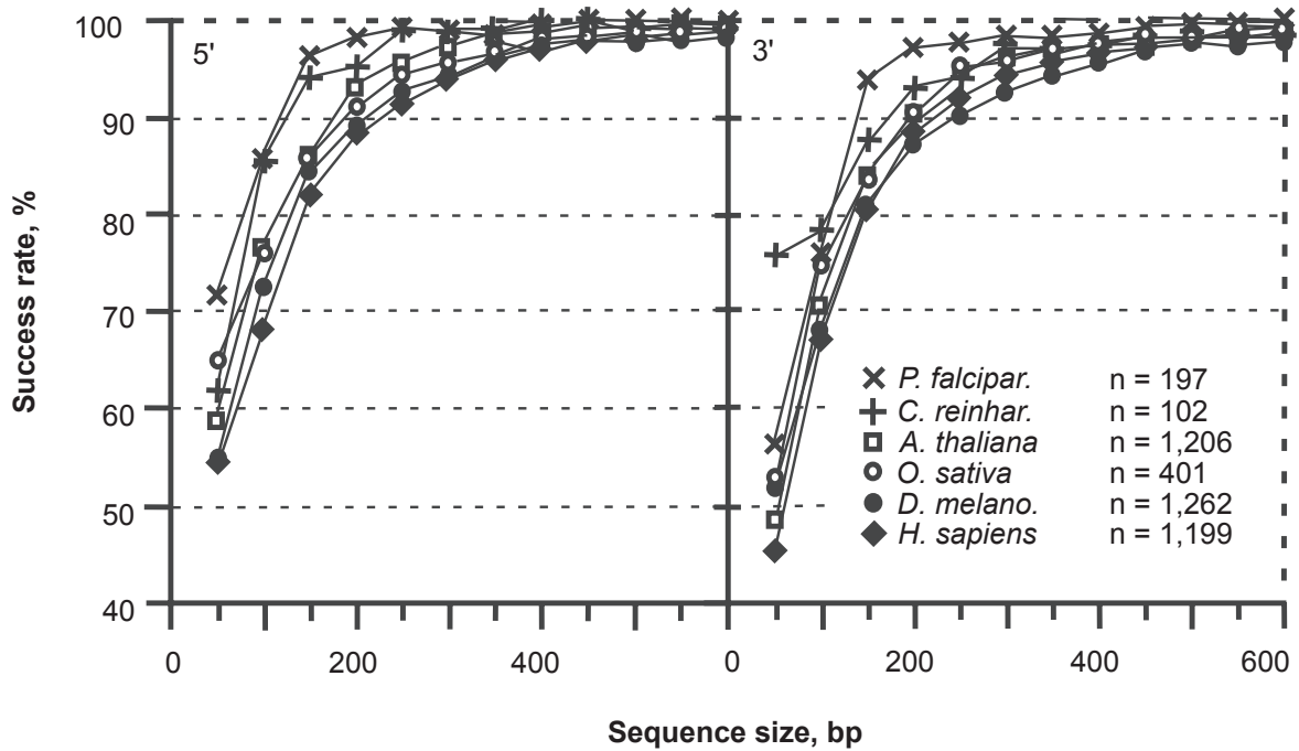
Figure 5. Classification of the coding frame among the six frames of coding sequences between 50 and 600 bp. The success rate of the function S=f_1+f_2 over six frames is shown for P. falciparum (X), C. reinhardtii (+), A. thaliana (□), O. sativa (O), D. melanogaster (●) and H. sapiens (◆), respectively.
