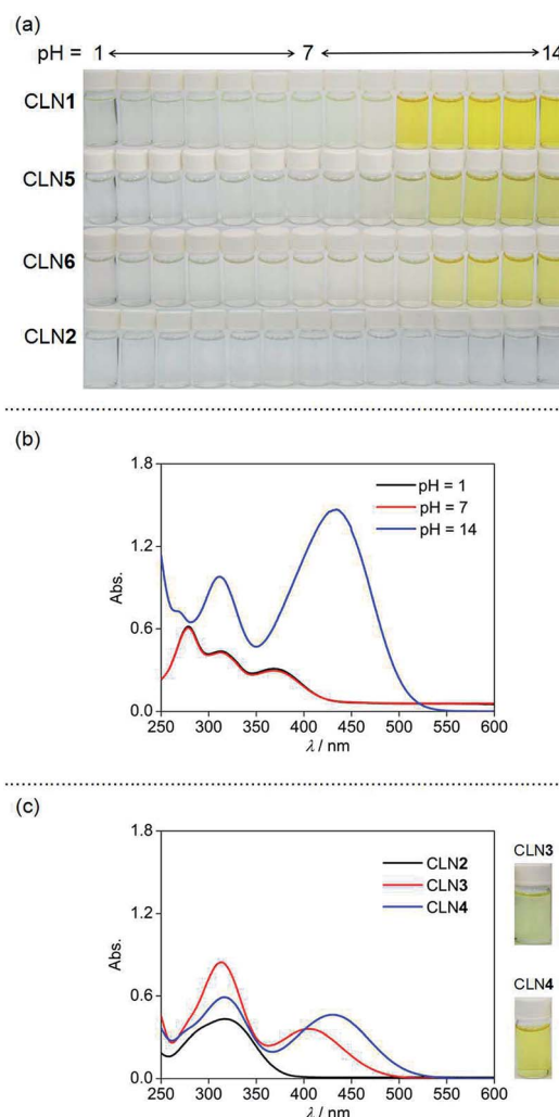
Fig. 2 (a) The pH dependent color changes of CLN1, 2, 5, and 6 in water ( \text{pH} = 1 –14). (b) The UV-vis absorption spectra of CLN1 at 298 K in water with \text{pH} = 1, 7 and 14. (c) The UV-vis absorption spectra of CLN2, 3, and 4 at 298 K in water with \text{pH} = 14 . The sample solutions were prepared upon fifty times dilution of a \text{CH}_3\text{CN} solution of CLN1–6 in volume with water. [\text{CLN}] = 4.0 \times 10^{-5} \text{ mol L}^{-1} .
