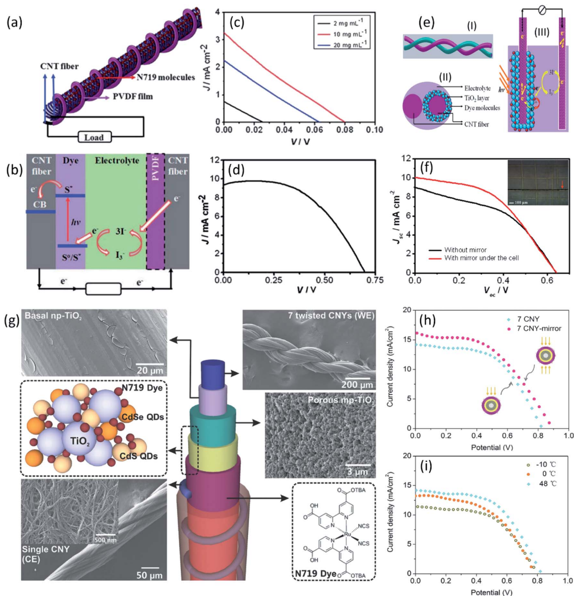
Fig. 2 (a) Schematic of a photovoltaic wire with two twined CNT fibers as working and counter electrodes, respectively. (b) The working principle of the photovoltaic. (c) J-V curves of photovoltaic wires using CNT/PVDF fibers prepared with different PVDF concentrations as counter electrodes and CNT/N719 composite fiber as working electrode. (d) J-V curve using aligned titanium dioxide nanotubes on Ti wire as the working electrode. 58 Copyright 2012, Royal Society of Chemistry. (e) Schematic illustration and working mechanism of a wire-shaped DSSC fabricated from two CNT fibers. (f) J-V curves of a 1.1 cm long fiber cell without and with the use of a mirror, the inset illustrates a fiber cell being woven into a textile composed of aramid fibers. 59 Copyright 2012, American Chemical Society. (g) 3D wire-shaped DSSC using a platinumized CNT fiber as counter electrode, a braid of 7-twisted CNT fibers with hybrid coatings as the working electrode. (h) J-V curves of wire-shaped hybrid cell with and without a mirror beneath. (i) J-V curves of wire-shaped hybrid cells with different temperature. 60 Copyright 2014, Wiley-VCH.
