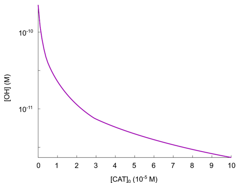
Figure 5. Maximal concentration of hydroxyl radicals as a function of catalase concentration in the regime 0 \leq [\text{CAT}]_0 \lesssim 10^{-4} M.
