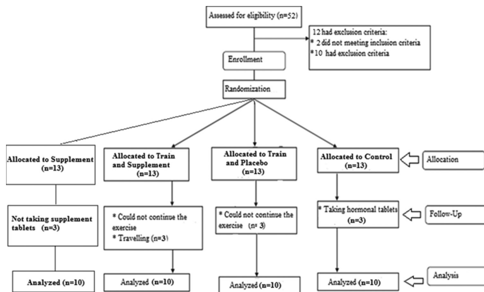
Figure 1: Consort flow diagram of the study
