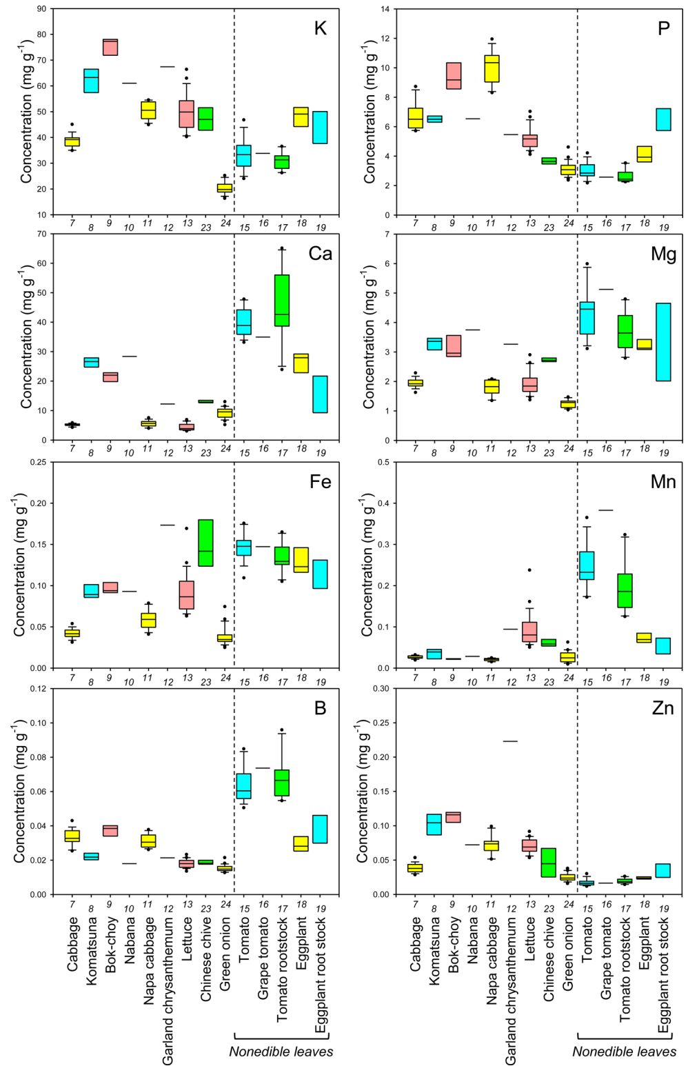
Fig 1. Boxplots showing the concentration of K, P, Ca, Mg, Fe, Mn, B, and Zn in leaves of various crop species. Concentrations in nonedible leaves are also shown. Numbers in x-axis indicate the species number in Table 1.
