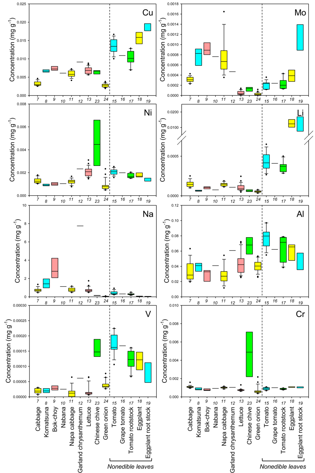
Fig 2. Boxplots showing the concentration of Cu, Mo, Ni, Li, Na, Al, V, and Cr in leaves of various crop species. Concentrations in nonedible leaves are also shown. Numbers in x-axis indicate the species number in Table 1 .
