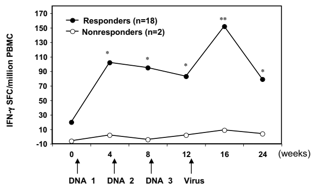
Figure 2 Antigen-specific IFN- \gamma responses against pre-erythrocytic antigen PfCSP . PBMC from PfCSP or CSLAM immunized monkeys (both PBS and CRL1005 formulations) were assayed against recombinant PfCSP protein by IFN- \gamma ELISpot. Results represent the mean net spot-forming cells (SFC) per million PBMC from all responders ( n = 18 ) (solid circle) or non-responders ( n = 2 ) (open circle) at the defined time points. DNA_1 = 1 st DNA immunization; DNA_2 = 2 nd DNA immunization; DNA_3 = 3 rd DNA immunization; Virus = ALVAC- Pf7 boost. Net SFC was calculated by correcting the SFC responses with antigen for background SFC without antigen. IFN- \gamma ELISpot responses were classified as positive if (1) the net SFC (mean SFC in experiment antigen wells – mean SFC in medium wells) was > 25 SFC per million PBMC, and (2) the stimulation index (ratio of mean SFC in experimental peptide wells to mean SFC in medium wells) was > 2 . (* p < 0.05 and ** p < 0.01 ).
