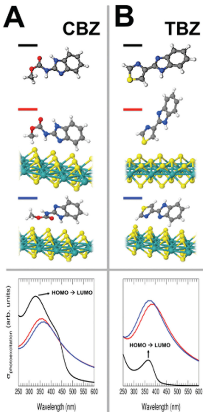
Fig. 3. Pictorial views of the DFT-based optimized free and interfacial systems and computed TDDFT photoexcitation spectra for: (A) free CBZ molecule (black line) and the two most stable CBZ/MoS 2 interfacial configurations (red and blue lines); and (B) free TBZ molecule (black line) and the two most stable TBZ/MoS 2 interfacial configurations (red and blue lines).
