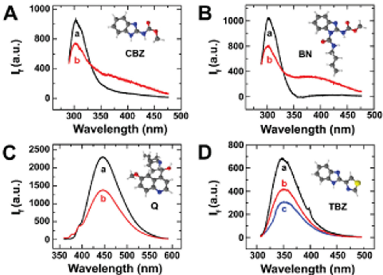
Fig. 2. Fluorescence emission spectra of (A) 2.50 \mu\text{M} CBZ, (B) 2.00 \mu\text{M} BN and (C) 0.500 \mu\text{M} Q in the absence (curve a) and in the presence (curve b) of \text{MoS}_2 90 nm. \lambda_{\text{exc}} = 280 nm (CBZ and BN), 445 nm (Q). (D) 100 nM TBZ before (curve a) and after (curve b) the addition of GOx and (curve c) addition of \text{MnO}_2 . \lambda_{\text{exc}} = 294 nm.
