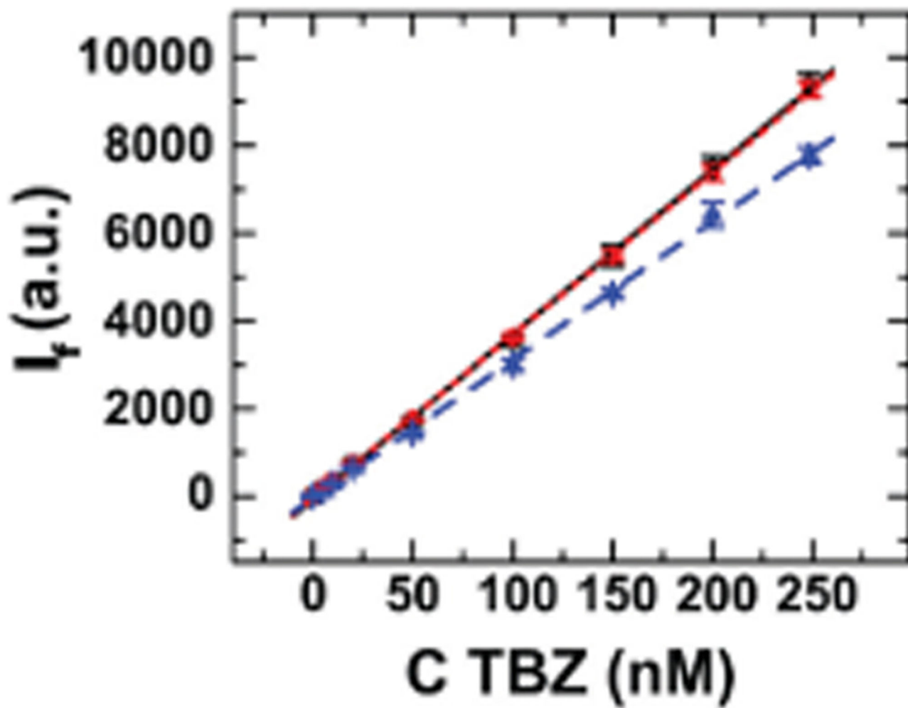
Fig. 5. Calibration curves of TBZ with 200 \mu L (black squares, solid line), 100 \mu L (red circles, dotted line) and 50 \mu L (blue triangles, dashed line) of WS 2 90 nm, 7.5 mg mL -1 in EtOH: H 2 O (45: 55, v/v). \lambda_{exc} = 294 nm; \lambda_{em} = 350 nm.
