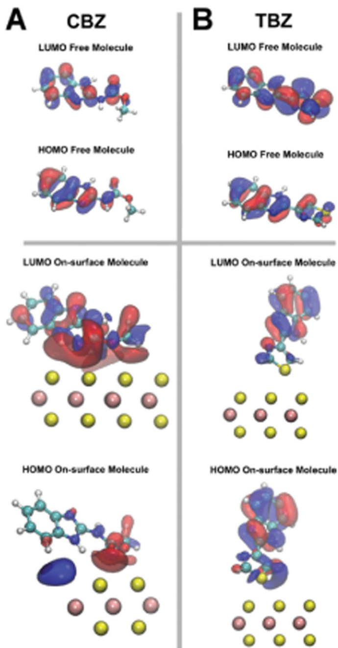
Fig. 4. Computed iso-surfaces at 0.05 \text{ e}^{-\text{\AA}^{-3}} of molecular orbitals for: (a) HOMO and LUMO of free CBZ, and molecular HOMO and LUMO of CBZ on \text{MoS}_2 , and (b) HOMO and LUMO of free TBZ, and molecular HOMO and LUMO of TBZ on \text{MoS}_2 . Red and blue iso-surfaces correspond to positive and negative regions of the wave functions, respectively.
