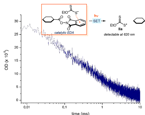
Figure 5. Absorption at 620 nm of the transient xanthyl radical IIa generated upon 355 nm laser excitation of a 1:1 mixture of 1a and catalyst B (30 mM) in DMA.
