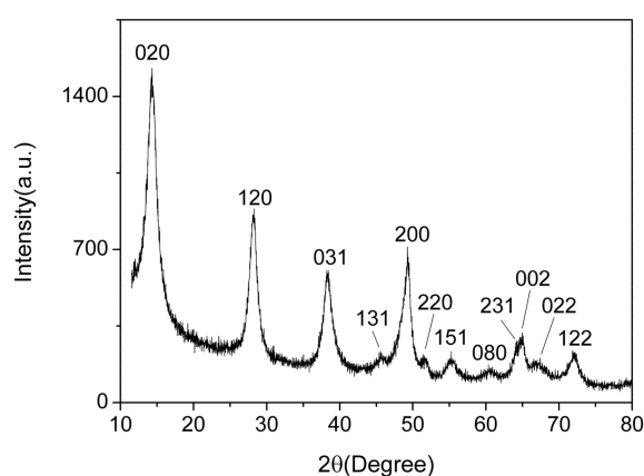
Figure 3. X-ray diffraction (XRD) of AlO(OH) film.
