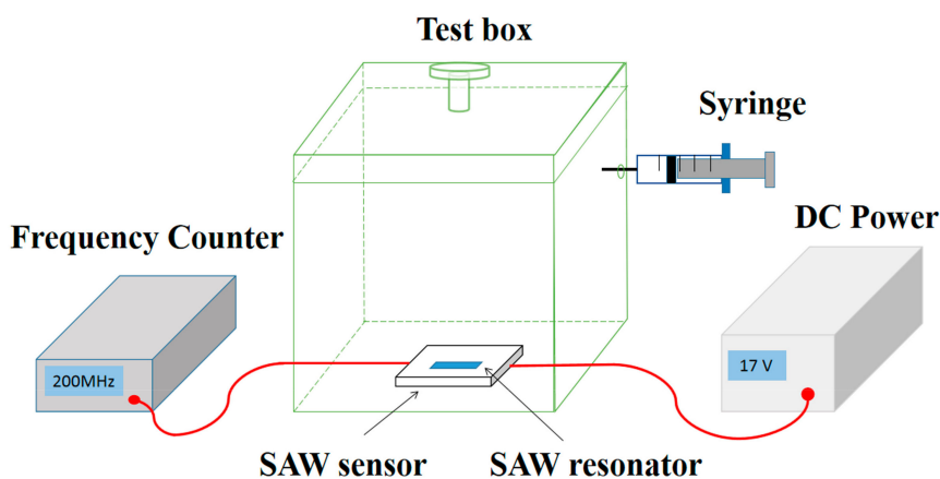
Figure 2. The experimental system of the gas-sensing test.
