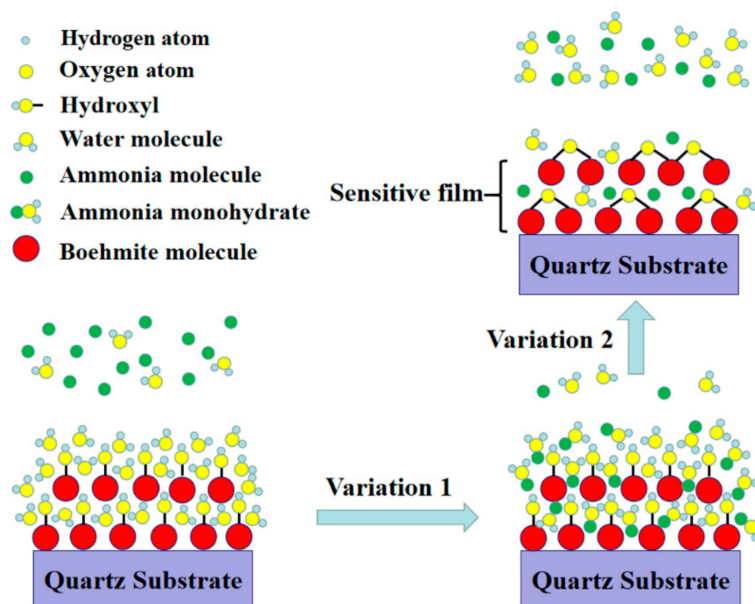
Figure 11. Sensing principle of \text{AlO}(\text{OH}) film with hydroxyl groups.
