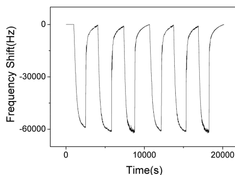
Figure 12. The dynamic response and recovery of SAW sensor with \text{AlO}(\text{OH}) film towards relative humidity change from 40% to 70% for 6 cycles.
