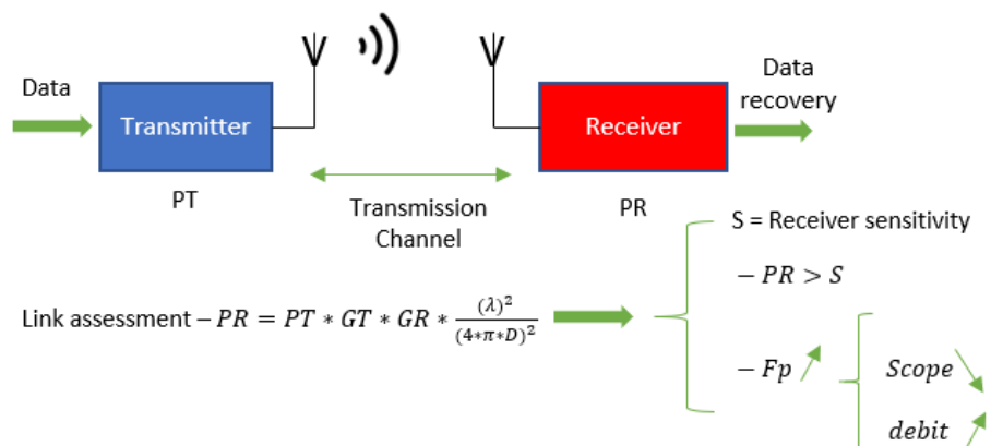
Figure 3. Link budget.
