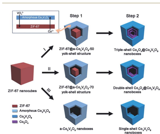
Fig. 4 A schematic diagram of the formation of complex \text{Co}_3\text{O}_4@ \text{Co}_3\text{V}_2\text{O}_8 hollow structures. Step 1 involves solvothermal reactions with different amounts of vanadium oxytriisopropoxide (VOT): (I) 50 \mu\text{L} , (II) 70 \mu\text{L} , and (III) 120 \mu\text{L} . Step 2 is simple annealing in air. Reproduced with permission. 54 Copyright 2018, Wiley-VCH.
