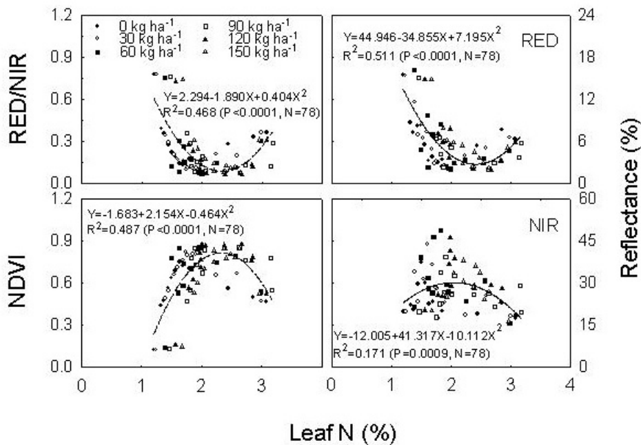
FIGURE 9. Correlation between reflectance at the red light minimum (RED), near-infrared peak (NIR), vegetation indices (RED/NIR ratio and NDVI), and leaf nitrogen content in rice plants grown under different nitrogen fertilizer application rates (0, 30, 60, 90, 120, and 150 kg ha -1 ) during the growing season of 2000.
