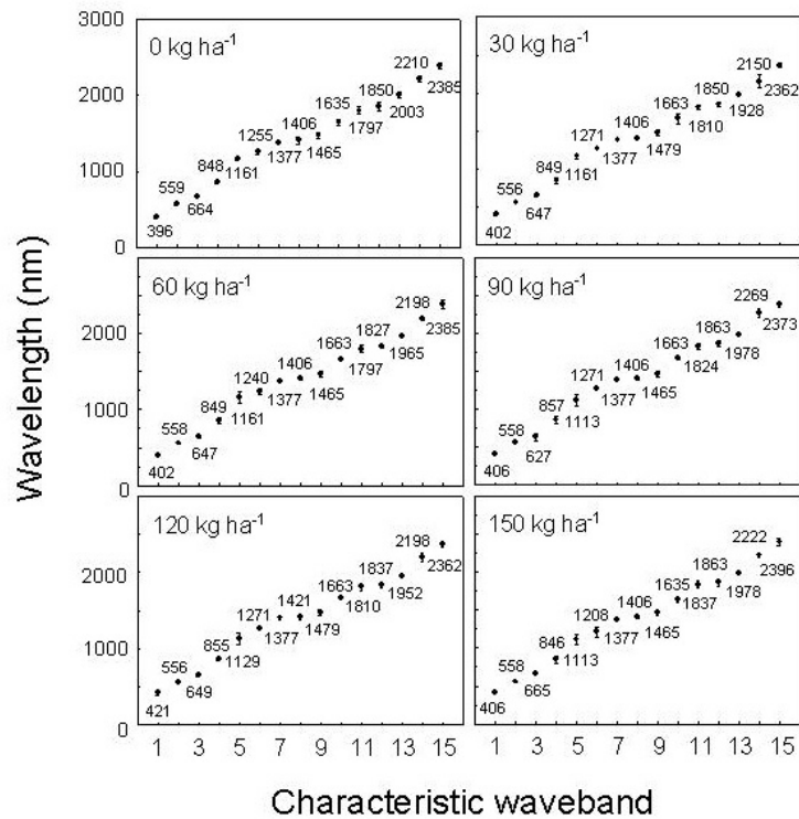
FIGURE 2. The center wavelengths and standard deviations of 15 characteristic wavebands selected from canopy reflectance spectra of rice plants grown under different nitrogen fertilizer application rates (0, 30, 60, 90, 120, and 150 kg ha -1 ) during the growing season of 2000.
