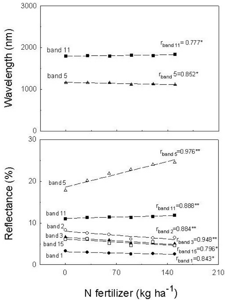
FIGURE 4. Wavebands and spectral reflectance identified from rice canopy reflectance spectra can be used to distinguish the affects of different nitrogen fertilizer application rates.
