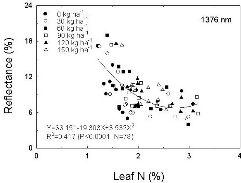
FIGURE 8. Correlation between reflectance and leaf nitrogen content at wavelength of 1376 nm in rice plants grown under different nitrogen fertilizer application rates (0, 30, 60, 90, 120, and 150 kg ha -1 ) during the growing season of 2000.
