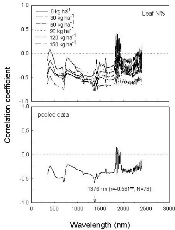
FIGURE 7. The correlation intensity curves of spectral reflectance to leaf nitrogen content in the range of 350-2400 nm in rice plants grown under different nitrogen fertilizer application rates (0, 30, 60, 90, 120, and 150 kg ha -1 ) during the growing season of 2000.
