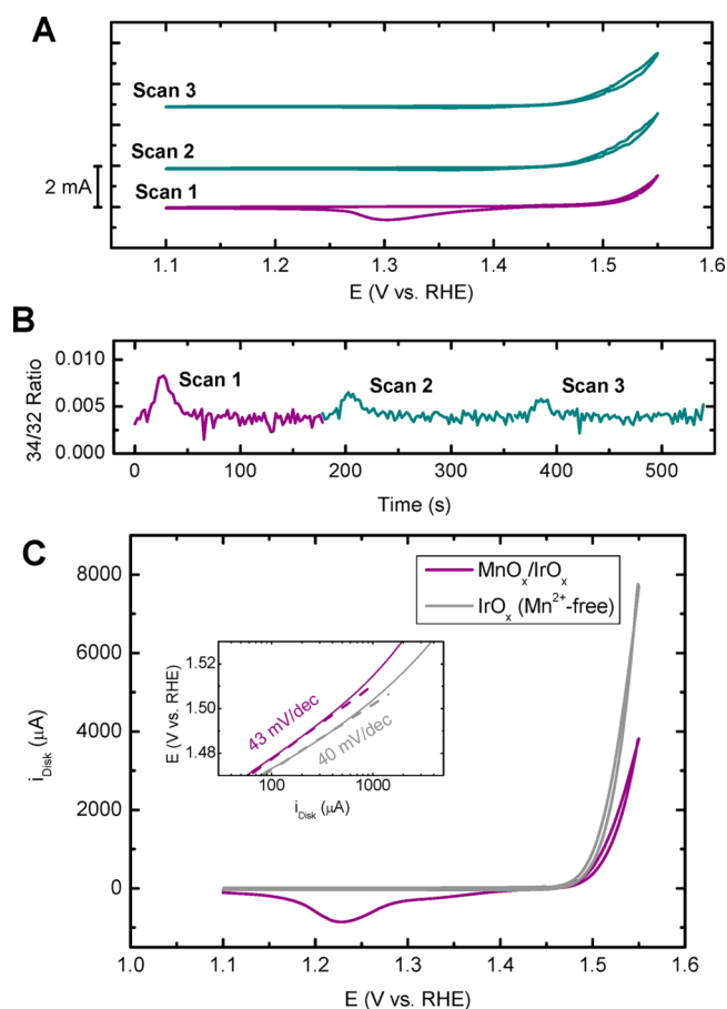
Figure 11. (A and B) OLEMS measurements of an “ \text{MnO}_x/\text{Ir}^{18}\text{O}_x/\text{GC} ” electrode in 0.5 M \text{KHSO}_4 , 30 mM \text{KCl} , and 1.2 mM \text{MnSO}_4 (pH = 0.87). The isotopic labeling procedure is described in the text. The electrode was scanned three times (A), while monitoring the mass/charge ratio 34/32 (B). Scan rate: 5 \text{ mV s}^{-1} . (C) CVs of an \text{IrO}_x/\text{GC} rotating disk electrode in 0.5 M \text{Na}/\text{HClO}_4 (pH = 0.85), in a \text{Mn}^{2+} -free solution (gray) and in the presence of 0.6 mM \text{Mn}(\text{ClO}_4)_2 with a preconditioned \text{MnO}_x film before initiating the forward scan at 1.45 V (purple). Inset shows calculated Tafel slopes determined from forward–backward averaged disk currents. Scan rate: 10 \text{ mV s}^{-1} ; rotation rate: 1500 rpm. All solutions are saturated with Ar.
