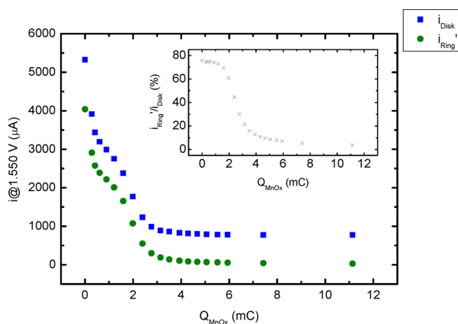
Figure 3. Disk (blue) and ring currents (green) measured at E_{\text{Disk}} = 1.55 \text{ V} as a function of Q_{\text{MnO}_x} , the reductive charge measured for the corresponding \text{MnO}_x film during the backward scan, which is an approximate measure of its thickness. Inset shows the ratio between i_{\text{Disk}} and i_{\text{Ring}} corrected for N_l ( i_{\text{Ring}}' ). Values were determined from CVs such as those in Figure 2.
