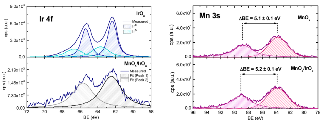
Figure 10. Core-level XPS scans of the Ir 4f (left) and Mn 3s (right) spectral peaks, on an absolute intensity scale. Both elements were scanned in samples of their \text{MO}_x/\text{GC} single oxides (top panels) and the mixed \text{MnO}_x/\text{IrO}_x/\text{GC} sample (lower panels). Note the difference in scale in the lower left-hand panel, illustrating the relatively low intensity of the Ir 4f signal.
