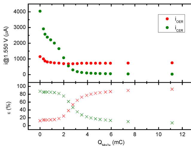
Figure 4. Top panel: currents for OER (red) and CER (green) at E = 1.55 \text{ V} , calculated from eq 3 and eq 7. Lower panel: corresponding selectivities toward OER (red) and CER (green). Data are plotted as a function of Q_{\text{MnO}_x} , the charge ascribed to the corresponding \text{MnO}_x layer, which is an approximate indication of its thickness. Values were determined from CVs such as those in Figure 2.
